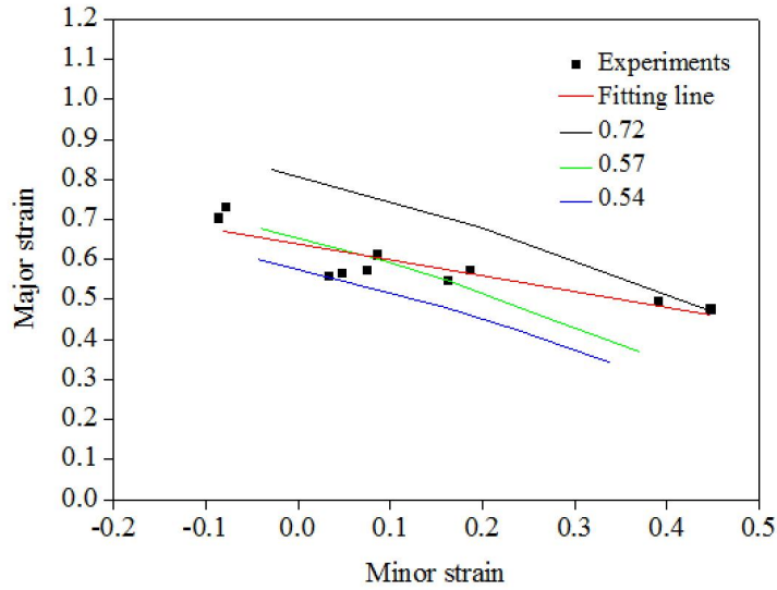
Figure 19: Prediction of forming limits with the Cockroft and Latham criterion, with different values of C1
