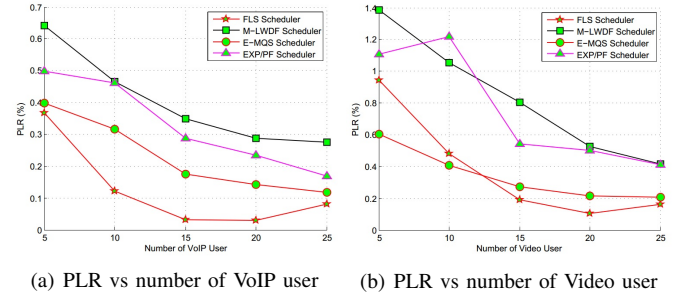
Fig. 2. Effects of PLR vs VoIP and Video users
