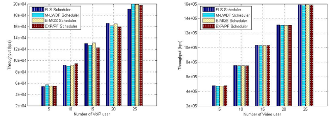
(a) Throughput vs number of VoIP user (b) Throughput vs number of Video user
