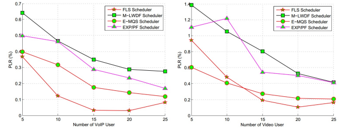
(a) PLR vs number of VoIP user (b) PLR vs number of Video user
