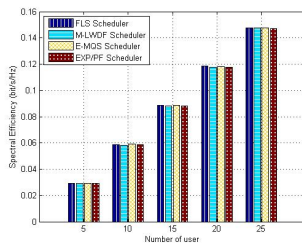
Fig. 5. Spectral efficiency vs number of user
