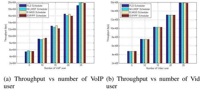
Fig. 3. Effects of Throughput vs VoIP and Video users
