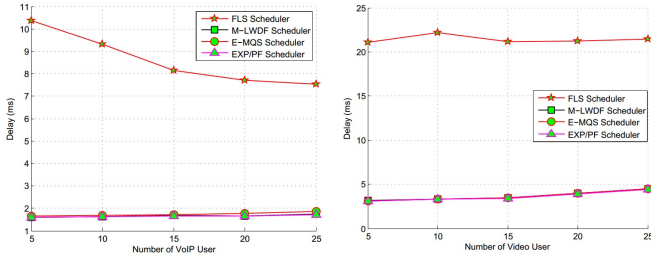
(a) Delay vs number of VoIP user (b) Delay vs number of Video user
