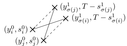
Fig. 2. An optimal permutation.
