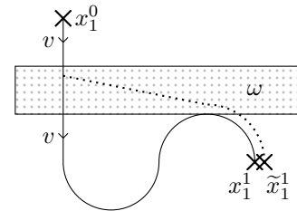
Fig. 1. Example of difference between t^1(x_1^1) and \bar{t}^1(x_1^1) .
