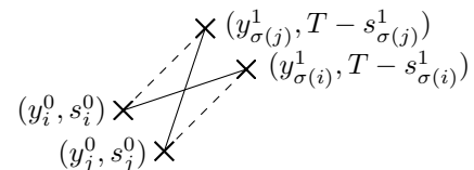
Fig. 2. An optimal permutation.
