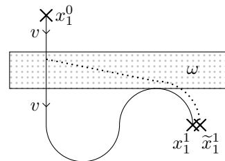
Fig. 1. Example of difference between t^1(x_1^1) and \bar{t}^1(x_1^1) .
