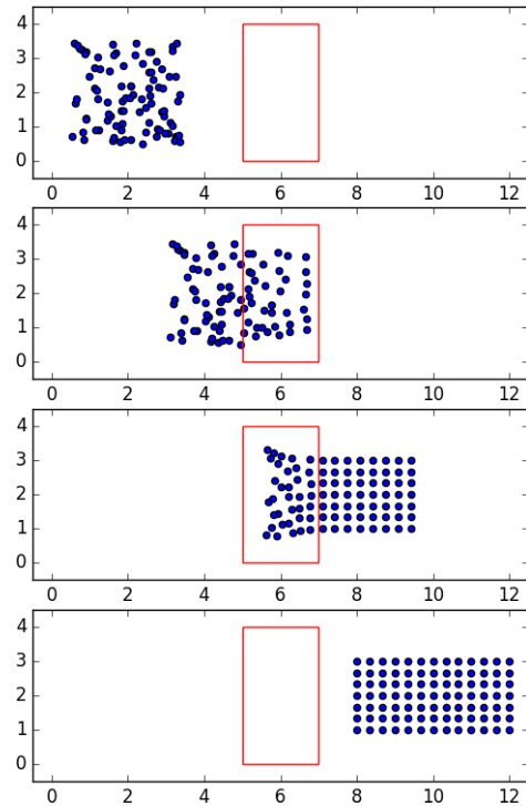
Fig. 4. Solution at time t = 0, t = 2.58, t = 5.18 and t = T = 7.75 .
