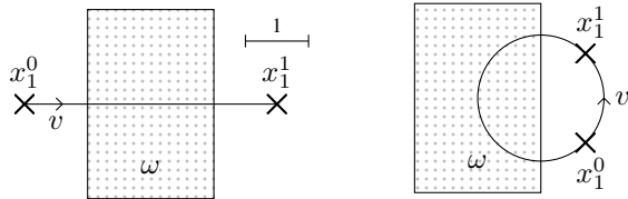
Fig. 3. Examples in the case T \in (0, M_e^*(X^0, X^1)) .
