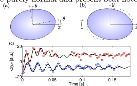
FIG. 1. (color online) Excitation of the scissors mode: (a) the trap axes are suddenly rotated by an angle \theta and (b) the gas starts oscillating around the new long trap axis. (c) Typical evolution of the observable \langle xy \rangle (average value of xy ), which is characteristic of the scissors mode. Red squares: thermal gas, two damped frequencies are present but no superfluid mode; blue triangles: superfluid oscillation of a well defined scissors mode.
