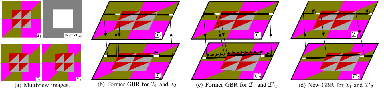
Fig. 2. GBR extensions to complex camera configuration. (a) Multiview images. From left to right and from top to bottom, the color images of \mathcal{I}_1 , the depth of \mathcal{I}_1 , the color images of \mathcal{I}_2 and \mathcal{I}'_2 . The camera displacements from \mathcal{I}_1 to \mathcal{I}_2 are only horizontal translations, while the displacements from \mathcal{I}_1 to \mathcal{I}'_2 are horizontal translations and rotations. In this example, \mathcal{I}_1 is reference view, while \mathcal{I}_2 or \mathcal{I}'_2 is predicted view. (b) The former GBR [14] is constructed for \mathcal{I}_1 and \mathcal{I}_2 . The white pixels in \mathcal{I}_2 are disocclusions while the white ones in \mathcal{I}_1 are occlusions. Each row of \mathcal{I}_2 can be reconstructed from \mathcal{I}_1 by following the graph edges. Since the camera displacement is simple and the disparity is horizontal, the graph edges are sparse. (c) A naive extension of the former GBR for \mathcal{I}_1 and \mathcal{I}'_2 . \mathcal{I}'_2 can be recovered from \mathcal{I}_1 by following the graph edges, however since the camera displacements are complex (the disparity is two-dimensional), the graph edges are denser than the ones in (b). (d) The proposed extension of GBR for \mathcal{I}_1 and \mathcal{I}'_2 , in which the edges connect a pair of straight segments (across two views). The graph edges are as sparse as the simple case handled by the former GBR in (b).
