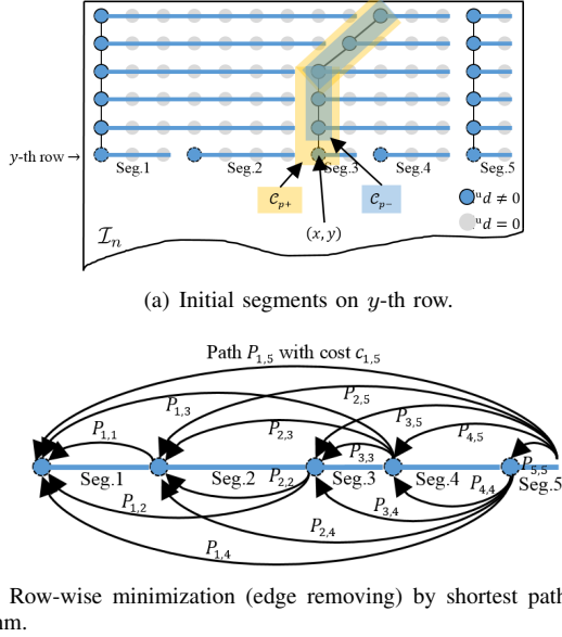
Fig. 8. Row-wise minimization. (a) Initialization. Pixels on y -th row have been grouped into five segments. Each segment has a constant depth. (b) Edge removing (segment merging). Some edges are removed (the segments are merged into their left neighboring segments) with respect to the row-base Lagrangian rate-distortion cost. The removing process is performed by shortest path minimization.
