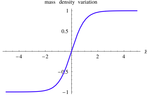
Figure 2: Classical density profile of the normalized density ( \tilde{\rho} \in ]-1, +1[ ) associated with (29) and (30); the x -axis unit is \ell .
