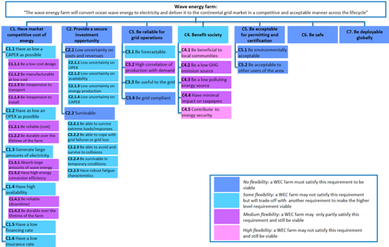
Figure 1: TPL Taxonomy
