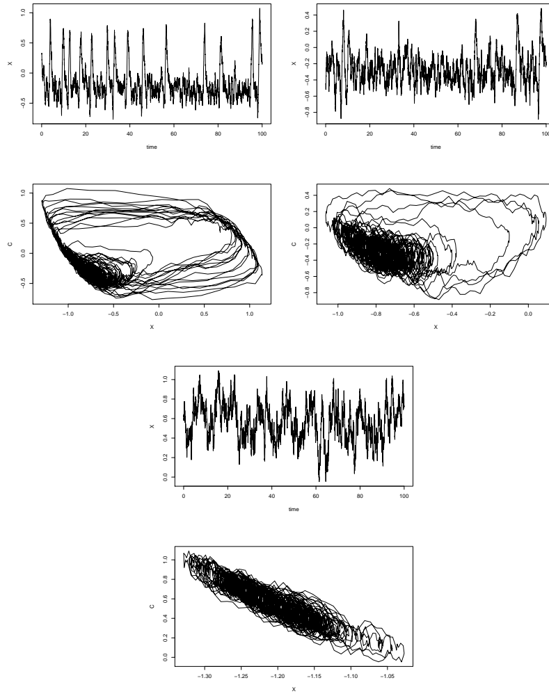
FIG 1. Simulations of the FitzHugh-Nagumo. Voltage variable X_t versus time (top line) and the corresponding trajectory in phase space C_t versus X_t (bottom line) for s = 0, \beta = 0.8, \bar{\sigma} = 0.3 , left: \varepsilon = 0.1 and \gamma = 1.5 , middle: \varepsilon = 0.4 and \gamma = 1.5 , right: \varepsilon = 0.5 and \gamma = 0.2 .
