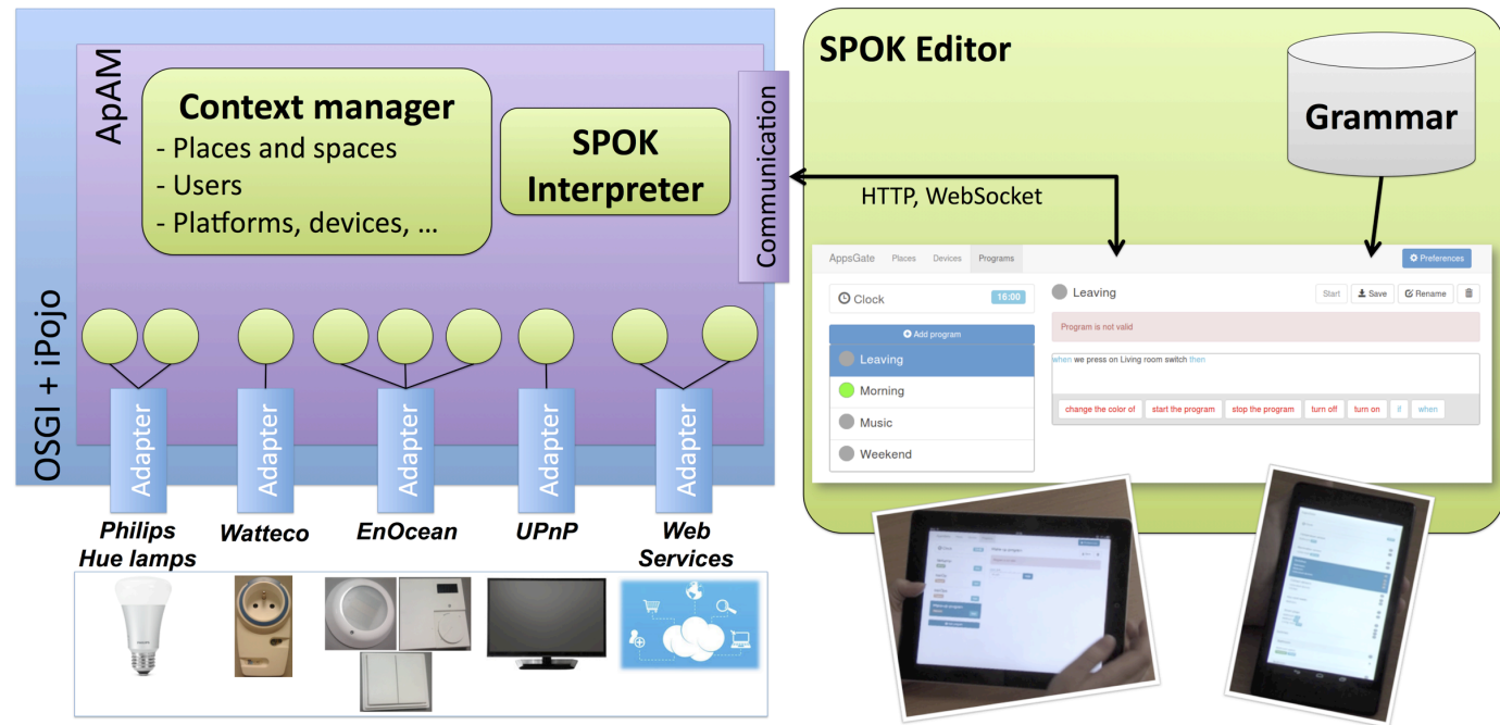
Figure 1. Overall software architecture of the Smart Home middleware on top of ApAM/OSGi-iPOJO and the SPOK editor running on client interaction devices (e.g., tablets, and Smart phones).
