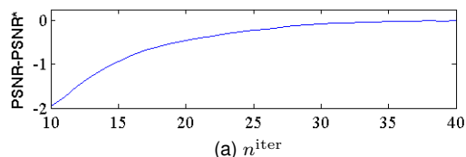
Fig. 10. Sensitivity analysis of parameters for Algorithm 3: median of psnr on 9 simulated images. The plots show the variations of PSNR when the parameters are moved around their optimal value on a range from half their value to twice their value. PSNR* corresponds to the PSNR of the optimum image found by the algorithms. The variations go up to 2dB, but vary very slowly after n^{\text{iter}} = 20 , our chosen value.
