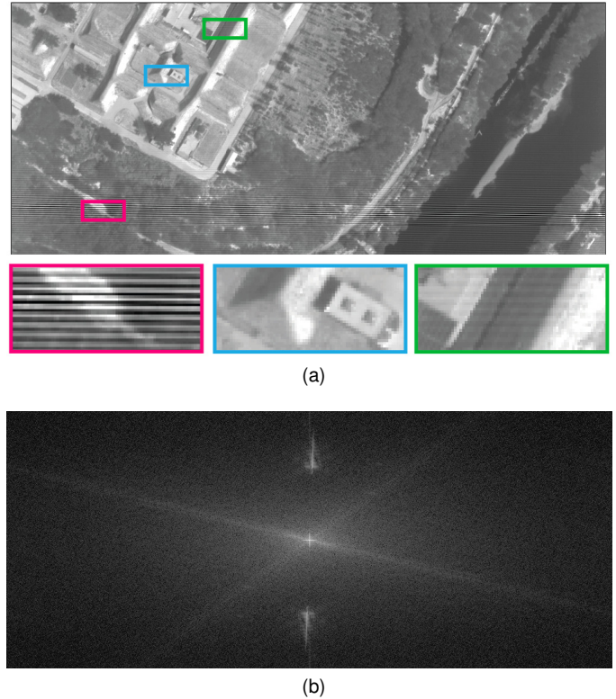
Fig. 1. On top, an image obtained with Sieteleters. Subimages are magnified to show the interference fringes overlaid on the scene. In red, an area with highly contrasted fringes. In blue, an area with blurred fringes. In green, an area with slightly contrasted fringes. The area with high contrast fringes is limited to the area around the zero optical path difference, due to the broadband observed spectra. Nonetheless, fringes are actually present over the whole image. Image (b) shows the Fourier spectrum of picture (a). The frequencies of the fringes are clearly seen as two very bright vertical lines. These frequencies constitute an area we call \Omega_0 .
