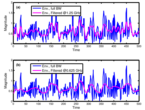
Fig. 3: Original envelope and reduced bandwidth envelope; (a) 1.25 GHz bandwidth (b) 625 MHz bandwidth
