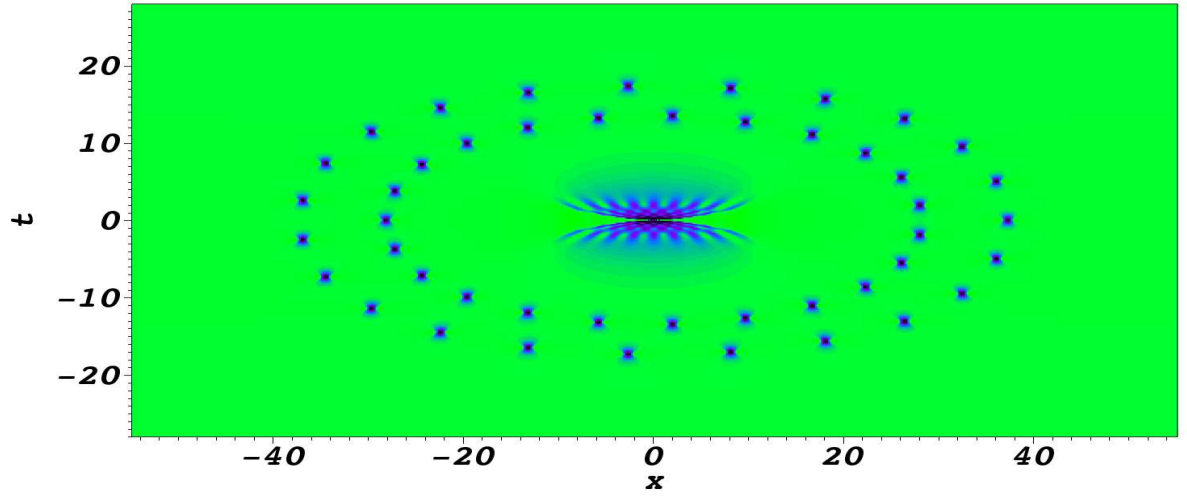
Figure 12: Solution to NLS, N=13 , a_{11} = 10^{20} : two rings with 23 peaks and in the center the Peregrine breather of order 9, sight from top.
