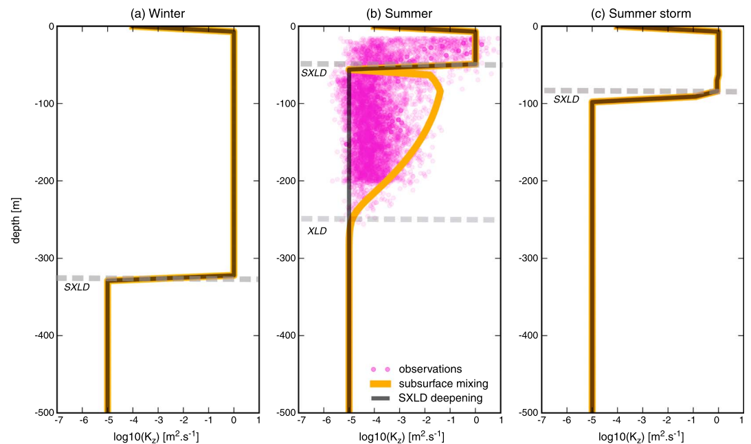
Figure 1. The prescribed k_z ( \text{m}^2 \text{s}^{-1} ) profiles of (a) winter, (b) summer (poststorm), and (c) during a summer storm. Two idealized cases: SXLD deepening (black) with slow mixing beneath the strong surface mixing and subsurface mixing with an enhanced gradient of mixing beneath the SXLD after summer storms (orange) and constrained summer k_z observations (magenta) in the ACC [Forryan et al. , 2015].
