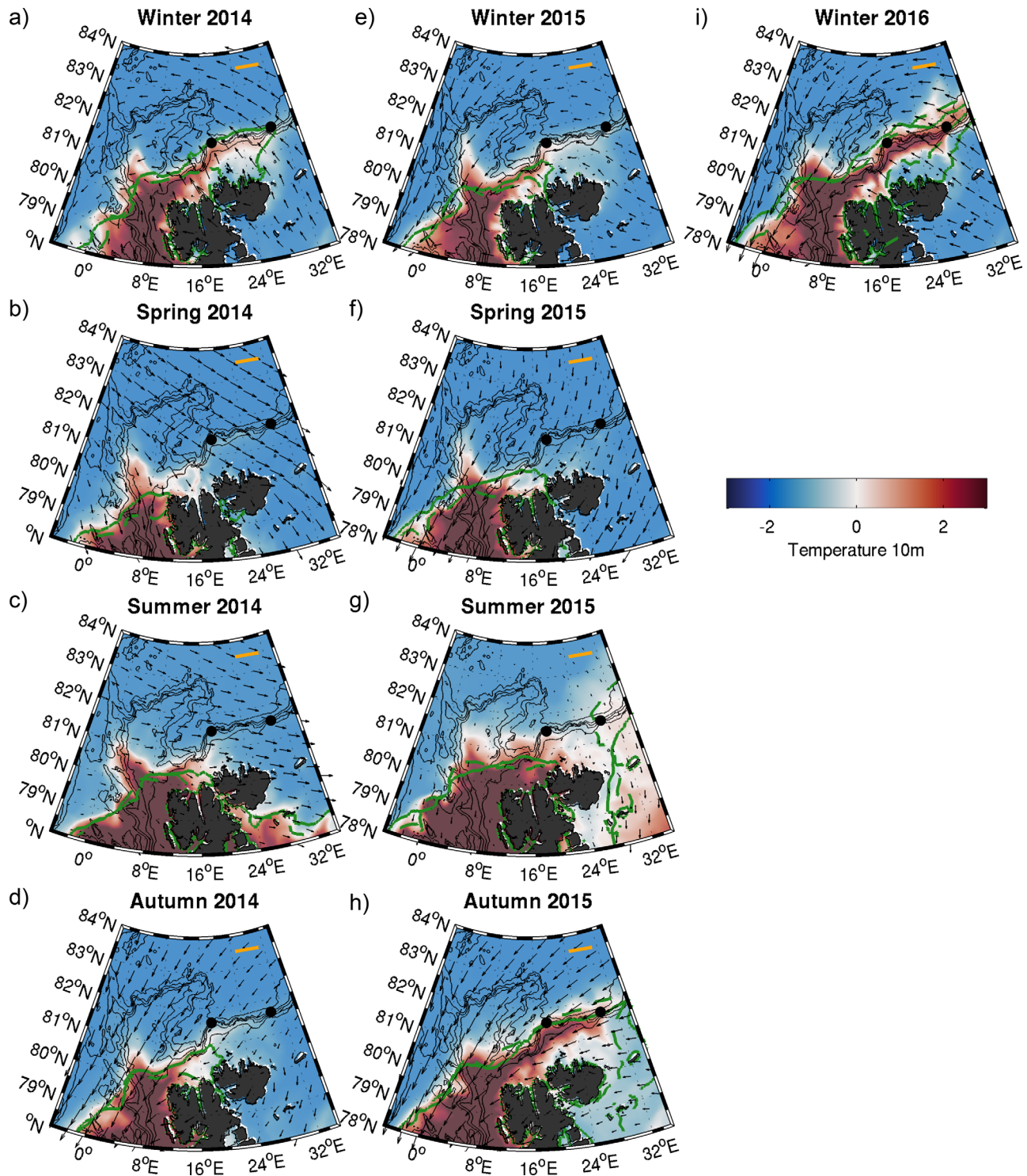
Figure 9. Wind speed at 10 m (arrows) averaged every 3 months from January 2014 to March 2016. (top right) The orange scale corresponds to 5 ms -1 . The green solid line (green-dashed line) is the 15% mean sea ice cover contour from AMSR-2 (model outputs) over the period and is taken as the location of the ice edge. The background color is the mean modeled ocean temperature at 10 m over the designated period. The thin black lines are the bathymetry contours. The black dots on the continental slope at 18°E and 30°E indicate the location of the shown profiles in Figure 12.
