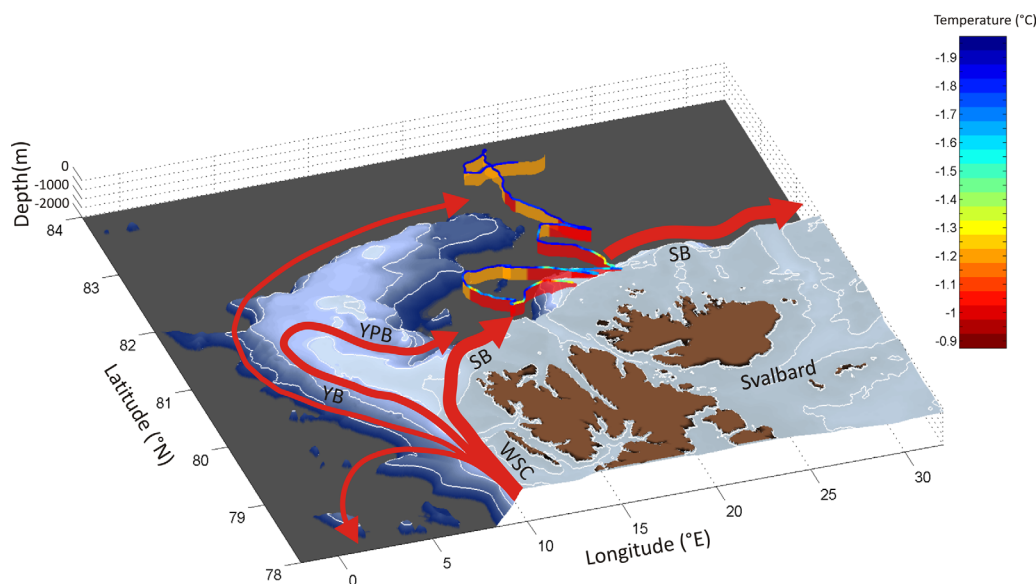
Figure 1. Summary of the in situ data results from Koenig et al. [2016] and Provost et al. [submitted]. The background of the 3-D plot is the bathymetry from IBCAO ( http://www.ngdc.noaa.gov/mgg/bathymetry/arctic/arctic.html ). The red lines are the warm water paths. YB: Svalbard Branch. WSC: West Spitsbergen Current. YPB: Yermak Pass Branch. SB: Svalbard Branch. Summary of the warm water layer is the orange/red ribbon: orange corresponds to Modified Atlantic Water and red to Atlantic Water. The overlaying data are the surface temperature obtained from the SIMBA instrument (colorbar on the side).
