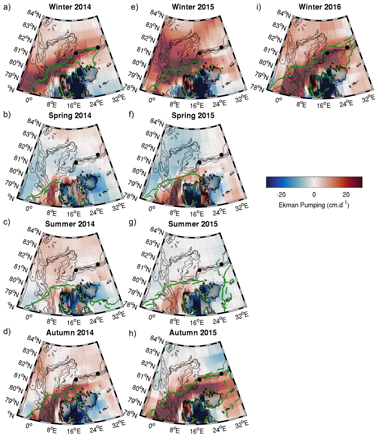
Figure 10. Ekman pumping ( \text{cm}\cdot\text{d}^{-1} ) averaged every 3 months from January 2014 to March 2016. The Ekman pumping is computed from the wind stress from ECMWF ( http://apps.ecmwf.int/datasets/data/interim-full-daily ). The green solid line (green-dashed line) is the 15% mean sea ice cover contour from AMSR-2 (model outputs) over the period and is taken as the location of the ice edge. The thin black lines are the bathymetry contours. The black dots on the continental slope at 18°E and 30°E indicate the location of the shown profiles in Figure 12.
