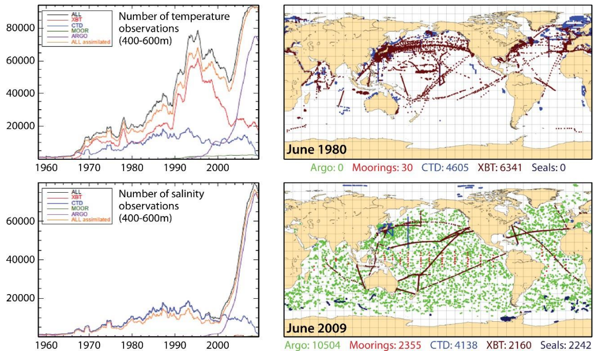
Figure 6 (left) Number of temperature (top) and salinity (bottom) observations within the depth range 400m-600m as a function of time per instrument type. The black curve is the total number of observations. The orange curve shows the number of assimilated observations. (Right) Observation coverage in June 1980 (top) and in June 2009 (bottom). Note that the colour coding for the instruments is not the same in the left and right panels. Data are as used in ORAS4. Source: ECMWF.
