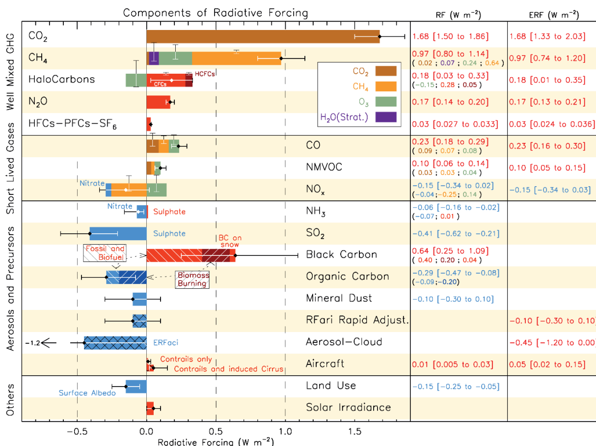
Figure 3 Radiative forcing ( Wm^{-2} ) of tropospheric climate change during the industrial era partitioned according to emitted compounds. The two sets of tabulated values in the right-hand columns differ due to differing extents to which conditions are held fixed in making the calculations of the changes in net radiative fluxes that result from changes in emissions over the era. Source: Stocker et al. (2013; Fig. TS.7), where further details may be found.
