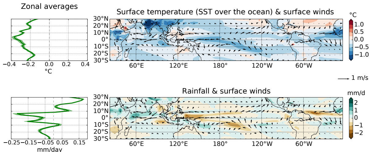
Fig. 2. MH-PI mean state differences. Right panel: MH-PI difference in the long-term mean surface temperature (SST over the ocean; top, ^\circ\text{C} ), rainfall (bottom, \text{mm/day} ) and surface winds (top & bottom, \text{m/s} ) in the tropical band. Left panel: zonal average of the surface temperature change (top, ^\circ\text{C} ) and of the rainfall change (bottom, \text{mm/day} ). Incertitude ranges on left panel give the 90% confidence intervals, estimated from bootstrap resampling (see Methods).
