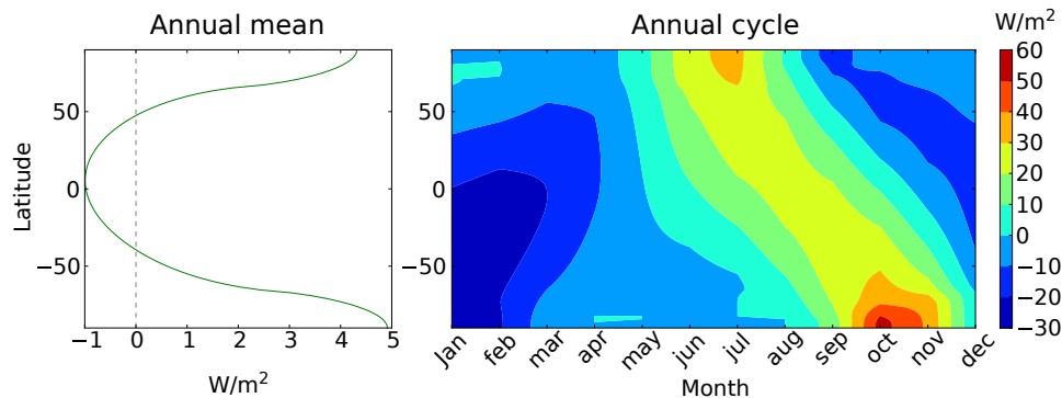
Fig. 1. Mid-Holocene insolation forcing. Left: MH-PI difference in the annual mean insolation (TOA incoming shortwave radiations) as a function of latitude ( W/m^2 ). Right: MH-PI difference in the mean annual cycle of insolation as a function of latitude ( W/m^2 ).
