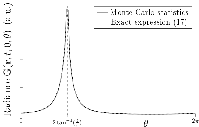
FIG. 2. Radiance for fixed \theta_0 = 0 , t = 1.1 and \mathbf{r} = (0, 1) (thus \theta_{\mathbf{r}} = \frac{\pi}{2} ) as a function of the propagation angle \theta . The Monte-Carlo simulations have been performed until 10^7 trajectories with at least two scattering events are found satisfying the fixed conditions for t and r within \Delta t = 0.05 and \Delta r = 0.05 . A total of 7.16 \times 10^{10} trajectories have been computed.
