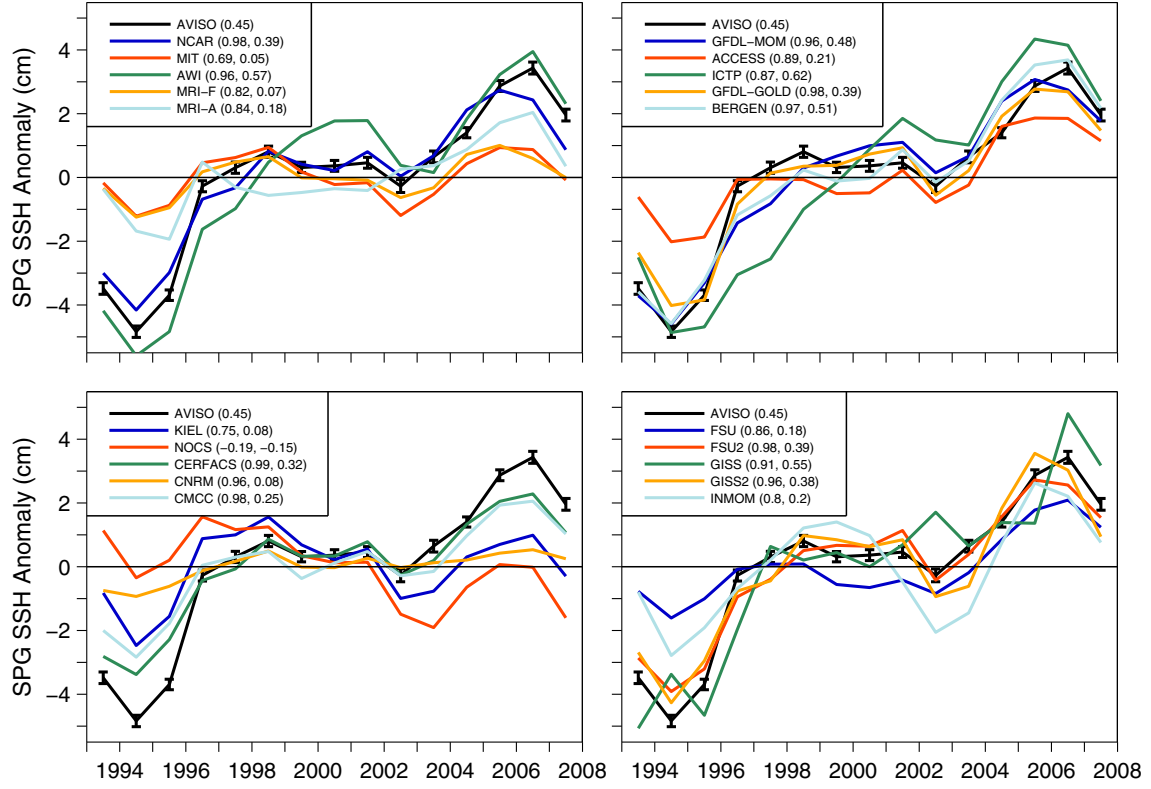
Figure 14: Time series of SPG SSH anomalies with respect to the 1993–2007 mean. SSH time series represent averages for the SPG region defined as the area between 15^{\circ} - 60^{\circ}\text{W} and 48^{\circ} - 65^{\circ}\text{N} . The SSH anomaly time series from AVISO dataset are also shown in each panel. The AVISO time series include the ranges of the spatially- and annually-averaged standard errors based on the monthly-mean data. The first number in parentheses for each model gives the correlation coefficient between the AVISO and that model's SSH time series. The second number in parentheses and the number for AVISO show the linear trend for the 1993–2007 period in \text{cm yr}^{-1} .
