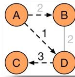
Figure 47. Same graph as figure 45 with a different MST
