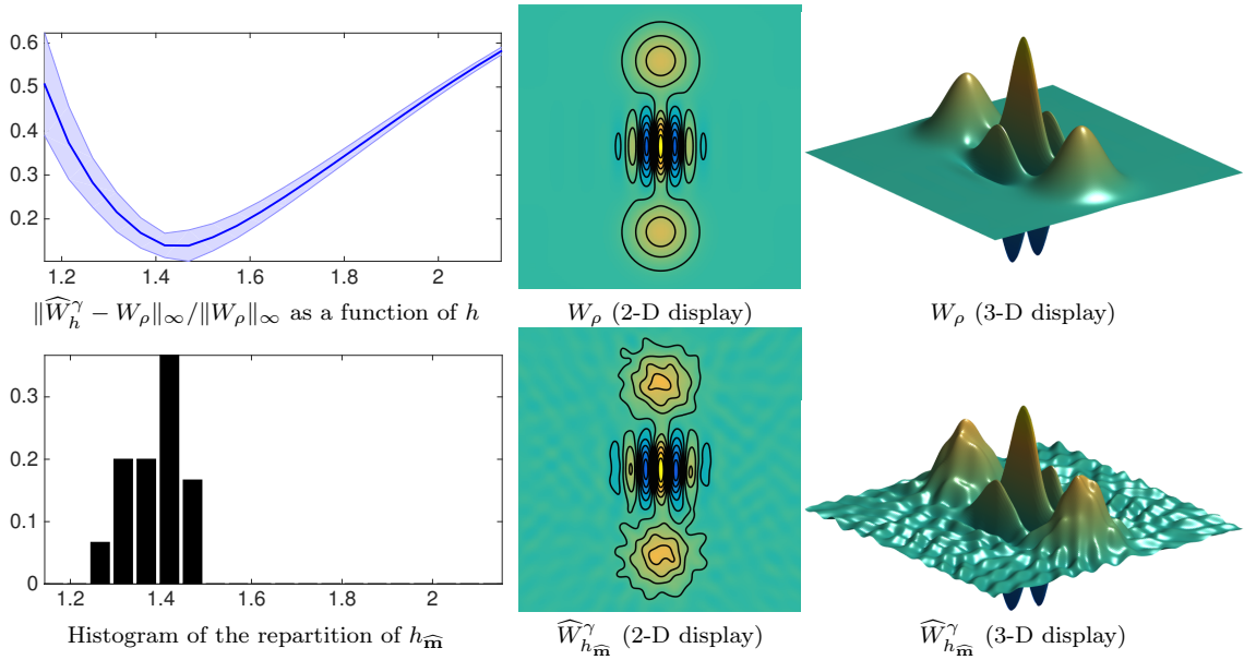
Figure 2: Schrödinger's cat state estimation, with \eta = 0.9 , n = 500 \times 10^3 . We refer to Figure 1 for the description of the plots.
