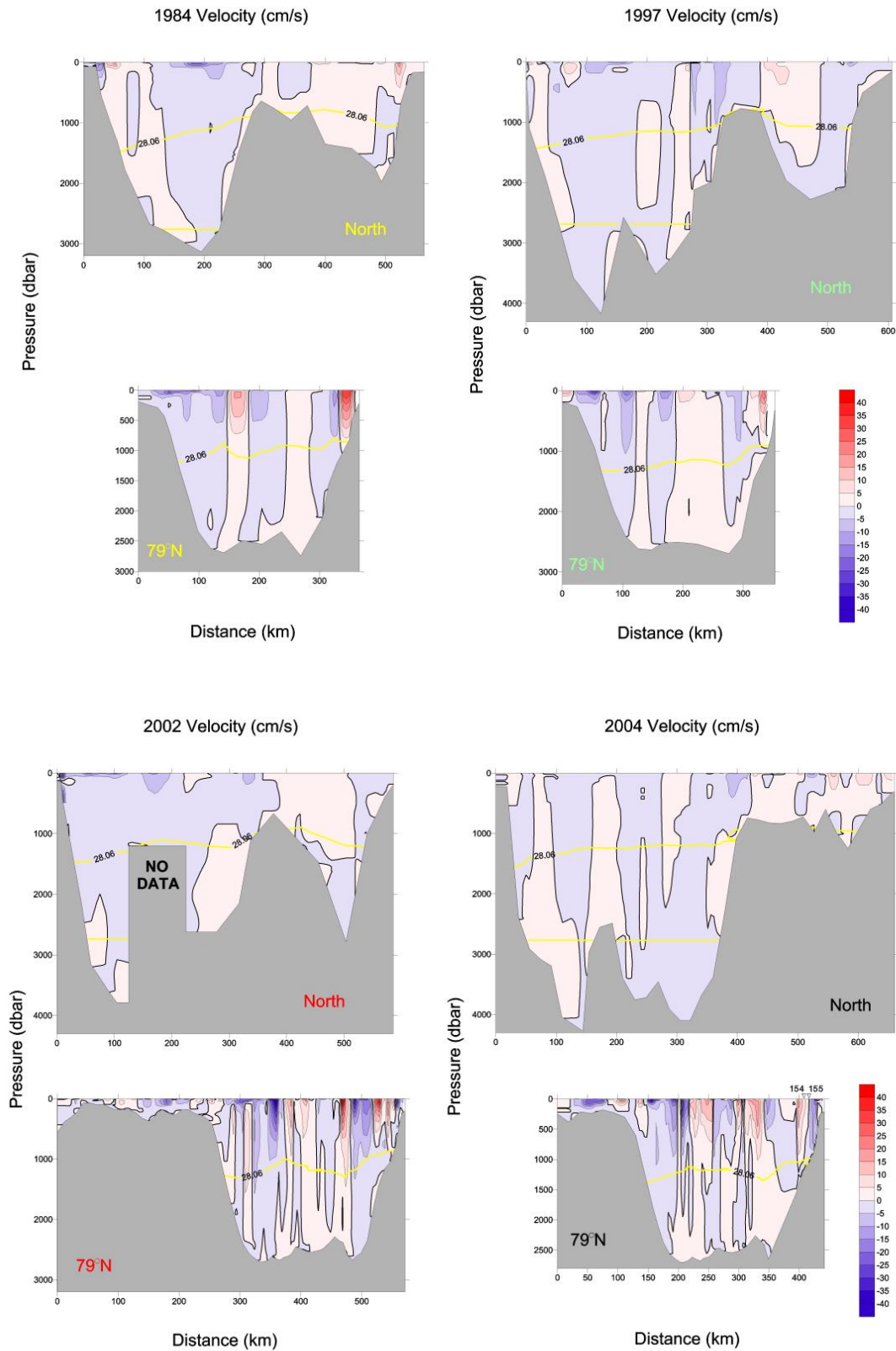
Fig. 3c. (a) Potential temperature, (b) salinity and (c) velocity with constraints applied from the zonal sections in 1984, 1997, 2002 and 2004 (Fig. 2). The constraint boundaries, potential density surface 28.06 and the 2744 dbar pressure level, are shown (yellow lines). Positive (negative) velocities are northward (southward). Stations 154 and 155 shown in Fig. 6 are marked with arrows in all the 2004 79° N sections. Colour coding of the sections (North for the northern section, and 79° N) follows that of Fig. 2.
