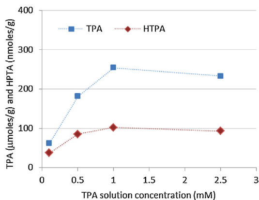
Fig. 5. HTPA ( \text{nmol g}^{-1} ) and TPA ( \mu\text{mol g}^{-1} ) content in TL as a function of TPA concentration in the impregnation solution.
