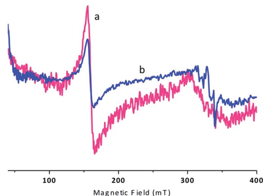
Fig. 4 EPR spectra of Extract 1 (a) and Extract 2 (b).
