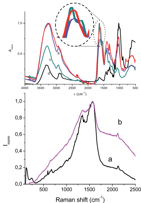
Fig. 2 Upper panel: IR spectra of Extract 1 (a, red), Extract 2 (b, purple), Extract 3 (c, green), and Whatman paper (d). The region around 1600\text{ cm}^{-1} is magnified to show the doublet of the green trace c. Lower panel: Raman spectra of Extract 1 (a) and Extract 2 (b).
