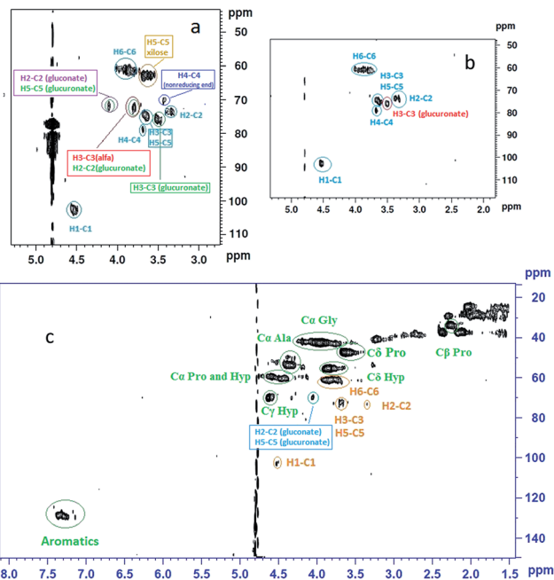
Fig. 3 HMQC spectra of Extract 1 (a), Extract 2 (b) and Extract 3 (c).
