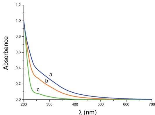
Fig. 1 UV-Vis spectra of Extract 1 (a), Extract 2 (b) and Extract 3 (c).
