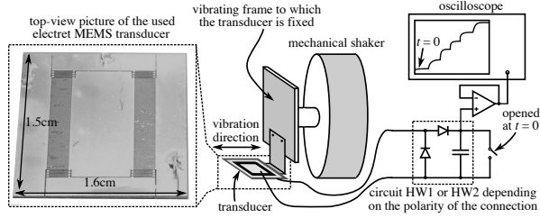
Fig. 3: Setup used for the measurement of the electret potential, with a top-view picture of the electret MEMS transducer. The device dimensions are 1.5\text{cm} \times 1.6\text{cm} \times 380\mu\text{m} .
