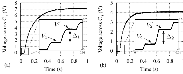
Fig. 2: Experimental measurement of (\Delta_1, \Delta_2, V_1, V_2) , measured on the MEMS electret transducer characterized in section III and reported in [10].
