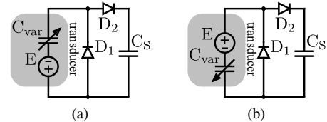
Fig. 1: Schematics of circuit HW1 (a) and circuit HW2 (b)
