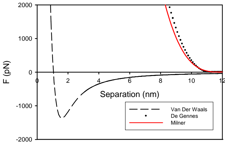
Fig.15 Comparison of the different forces between two particles coated by PPP44. Van der Waals :Eqs (4)-(5); De Gennes model: Eqs (4)-(5)-(8)-(9); Milner model: Eqs (4)-(5)-(7)-(9)
