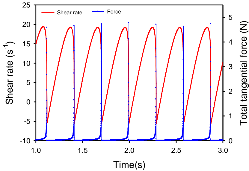
Fig19 In red the shear rate calculated for a viscoelastic liquid through Eqs (16)-(14) for a constant applied stress: \sigma_a=50\text{Pa} ; the shear modulus is given by Eq.(15) with G_0=3\text{Pa} and the parameter for the viscosity \eta_2 was \alpha=2 . In blue the total tangential force corresponds to the right axis.
