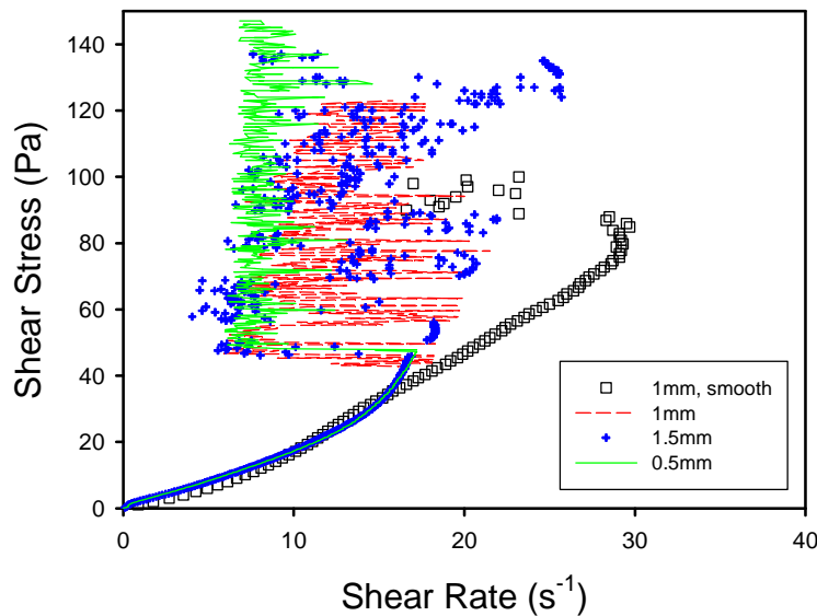
Fig.6 Three ramps of stress with different gaps: 0.5, 1, 1.5mm at \Phi=68\% with fluidizer PCP45 and serrated plates. The curve with open square symbols is obtained with smooth plates
