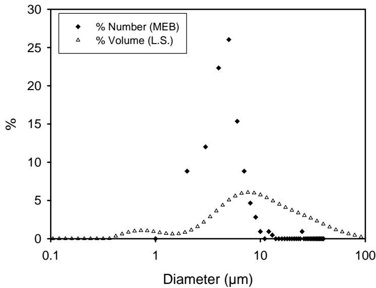
Fig.2 Size distribution obtained by counting the particles above 1µm from MEB pictures and from light scattering (L.S.) with Mastersizer 2000 from Malvern
