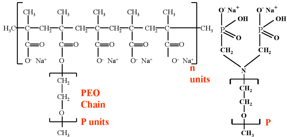
Fig. 3 Sketch of the two family of polymers. On the left PCP with a PEO chain of 45 or 114 units; on the right the PPP molecule with a PEO chain of 44 units
