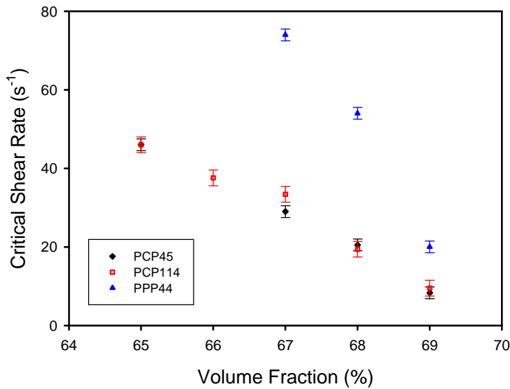
Fig.13 Evolution of the critical shear rate with the volume fraction for the three molecules
