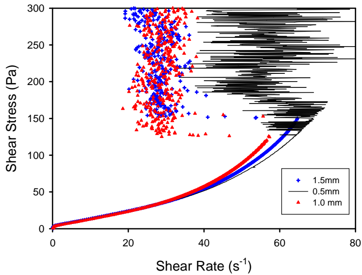
Fig.7 Three ramps of stress with different gaps and serrated plates at \Phi=68\% with fluidizer PPP44. The middle curve with crosses corresponds to 1.5mm
