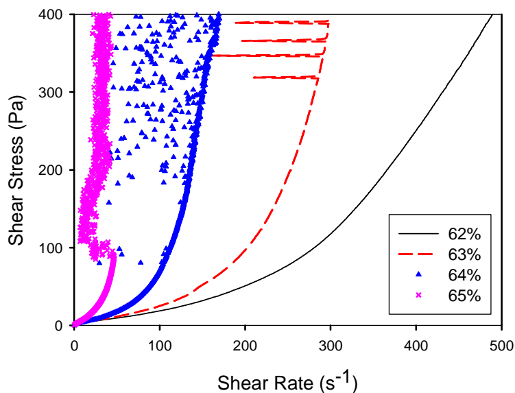
Fig.5 Evolution of the rheology of the suspension of calcium carbonate at different volume fractions adjuvanted with PCP45 at 0.2% wt. The increase of volume fraction goes from the right to the left
