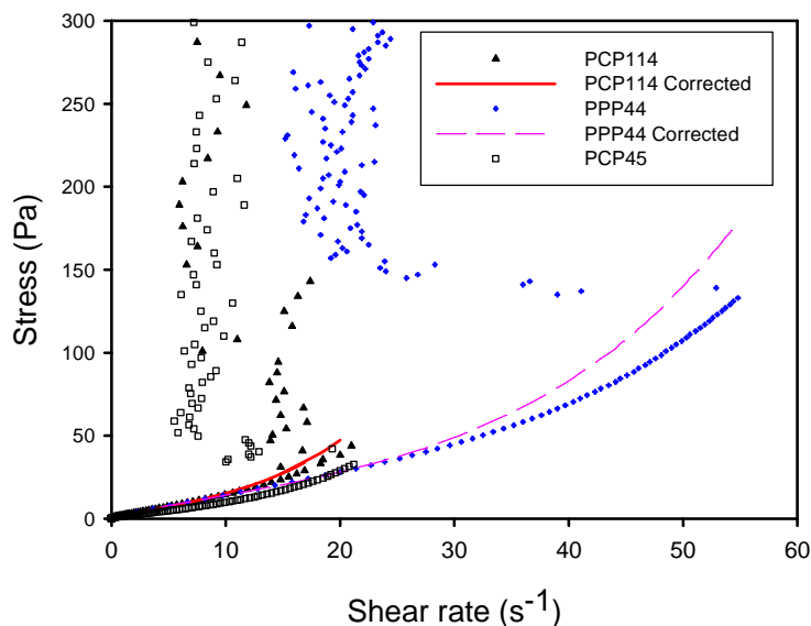
Fig.12 Comparison of the jamming transition for the suspension of \text{CaCO}_3 at \Phi=68\% for the three different molecules. The solid and dotted lines are obtained from Mooney-Rabinovitch correction
