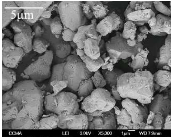
Fig.1. MEB view of calcium carbonate particles
