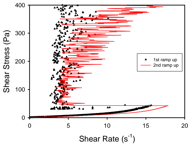
Fig.10 First and second ramp of stress for a suspension at \Phi=68\% with PCP45
