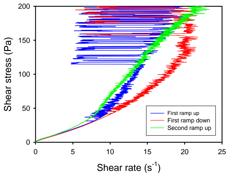
Fig.11 Same as Fig.10 but with the suspension extending outside the gap between the two plates
