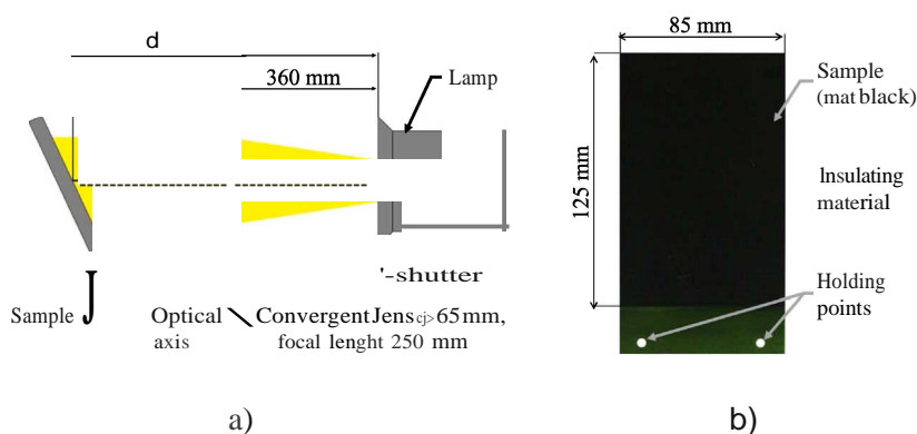
Fig.2. Optical system (a) and sample insulation on back-side (b).
