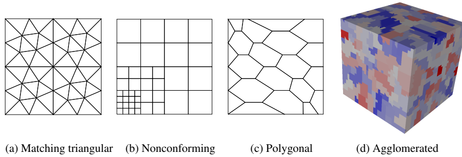
Fig. 1: Examples of polytopal meshes in two and three space dimensions. The triangular and nonconforming meshes are taken from the FVCA5 benchmark [31], the polygonal mesh family from [26, Section 4.2.3], and the agglomerated polyhedral mesh from [27].
