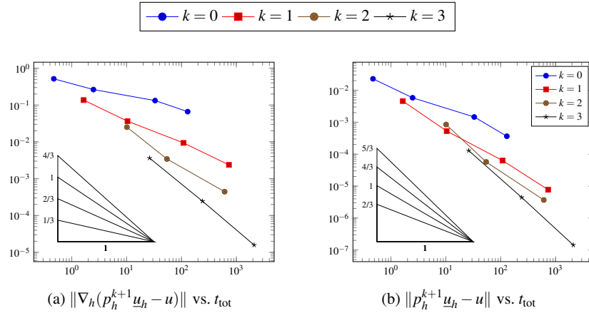
Fig. 6: Error vs. total computational time for the test case of Section 3.5.2.
