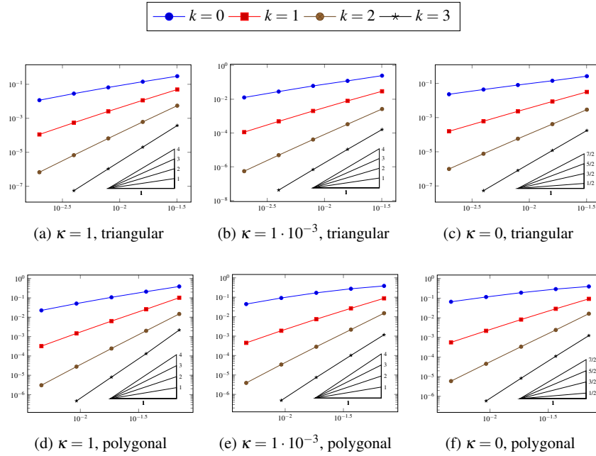
Fig. 9: \|L_h^k u - u_h\|_{\#,h} vs. h for the test case of Section 5.5.
