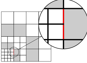
Fig. 2: Treatment of a nonconforming junction (red) as multiple coplanar faces. Gray elements are pentagons with two coplanar faces, white elements are squares.
