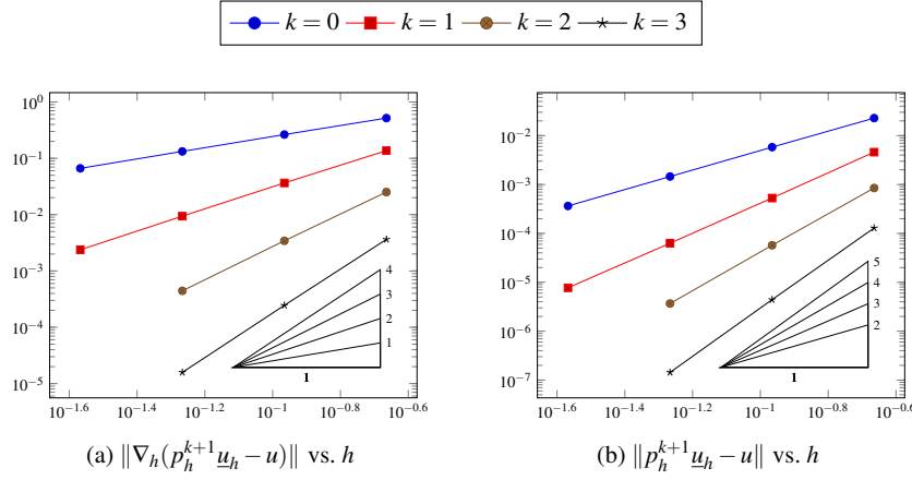
Fig. 5: Error vs. h for the test case of Section 3.5.2.
