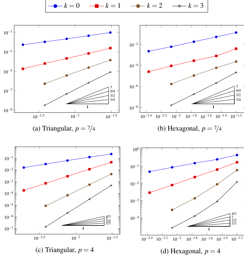
Fig. 8: \|I_h^k u - u_h\|_{1,p,h} vs. h for the test case of Section 4.5.
