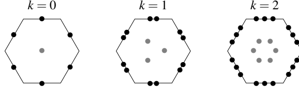
Fig. 3: DOFs in \underline{U}_T^k for k \in \{0, 1, 2\} . Internal DOFs (in grey) can be eliminated by static condensation (see Section 3.2.4).
