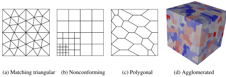
Fig. 1: Examples of polytopal meshes in two and three space dimensions. The triangular and nonconforming meshes are taken from the FVCA5 benchmark [31], the polygonal mesh family from [26, Section 4.2.3], and the agglomerated polyhedral mesh from [27].
