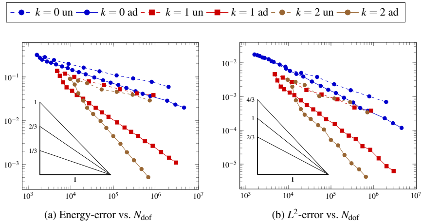
Fig. 7: Error vs. N_{\text{dof}} for the test case of Section 3.5.3.
