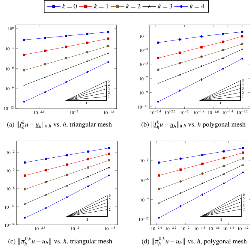
Fig. 4: Error vs. h for the test case of Section 3.5.1.
