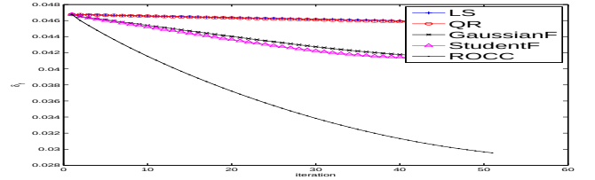
Fig. 5: Comparison of the relative error \|\hat{\mathbf{f}} - \mathbf{f}\|^2 / \|\mathbf{f}\|^2 of all the methods applying with the Walnut image with 180 projections.
