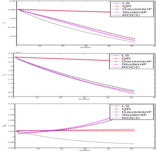
Fig. 3: Comparison of all the methods applying with the Shepp Logan image with 180 projections. These three figures, from top to bottom, show respectively the relative errors of the image \|\hat{\mathbf{f}} - \mathbf{f}\|^2 / \|\mathbf{f}\|^2 , the projections \|\hat{\mathbf{g}} - \mathbf{g}\|^2 / \|\mathbf{g}\|^2 and the contours \|\hat{\mathbf{f}} - \mathbf{f}\|^2 / \|\mathbf{f}\|^2 .
