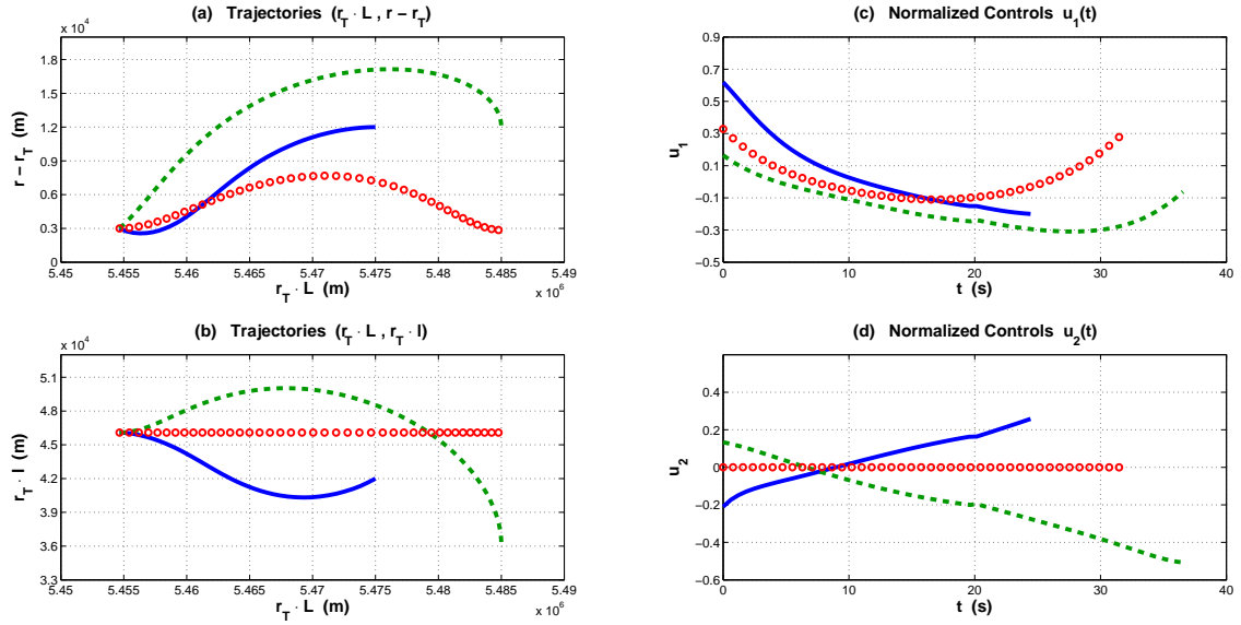
Fig. 1. Optimal trajectories and controls u_1, u_2 . The solid line represents \mathcal{S}_1 , while the dashed and the empty-dot lines represent respectively \mathcal{S}_2 and \mathcal{S}_3 .
