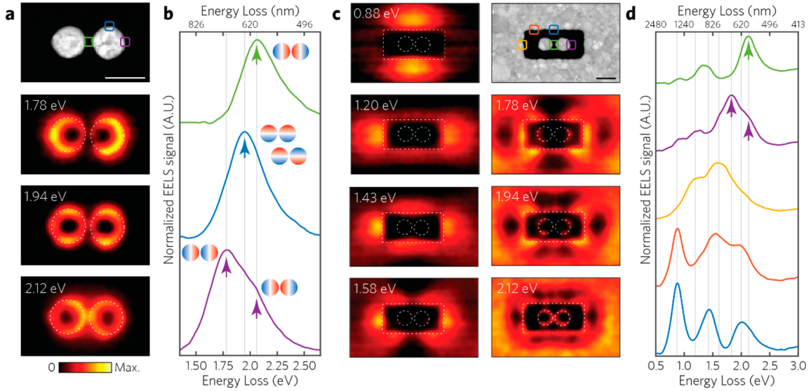
Figure 3. EELS analysis. (a) EELS maps at energy slices corresponding to the intensity maxima identified by extracting various spectra (b) at different impact parameters highlighted in the high-angle annular dark-field image, for an isolated dimer without surrounding box. The bonding and antibonding longitudinal dipoles are spatially and spectrally resolved at 1.78 and 2.12 eV, respectively. The bonding and antibonding transverse dipoles are revealed at 1.94 eV with a characteristic EELS signal distribution along the sides of the dimer. In the case of the antenna-in-box (c,d), low energy modes at 0.88 and 1.2 eV correspond to the fundamental dipole excited along the long or short axis of the rectangular box aperture, respectively. Multiple higher order harmonics are spatially and spectrally resolved from 1.43 eV and higher. The mode excited at 1.78 eV corresponds to the longitudinal bonding dipole of the dimer. A second mode, well identified in the green curve, corresponds to the expected higher energy (2.12 eV) antibonding longitudinal dipole. The EELS colormap is scaled to the data range of each map and scale bars are 100 nm.
