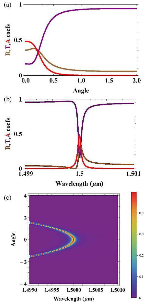
FIG. 5. (Color online) Reflection, transmission, and absorption coefficients as functions of (a) \theta at \lambda = 1.5 \mu\text{m} and (b) \lambda at \theta = 0 . (c) Mapping of the absorption coefficient in terms of \lambda and \theta .
