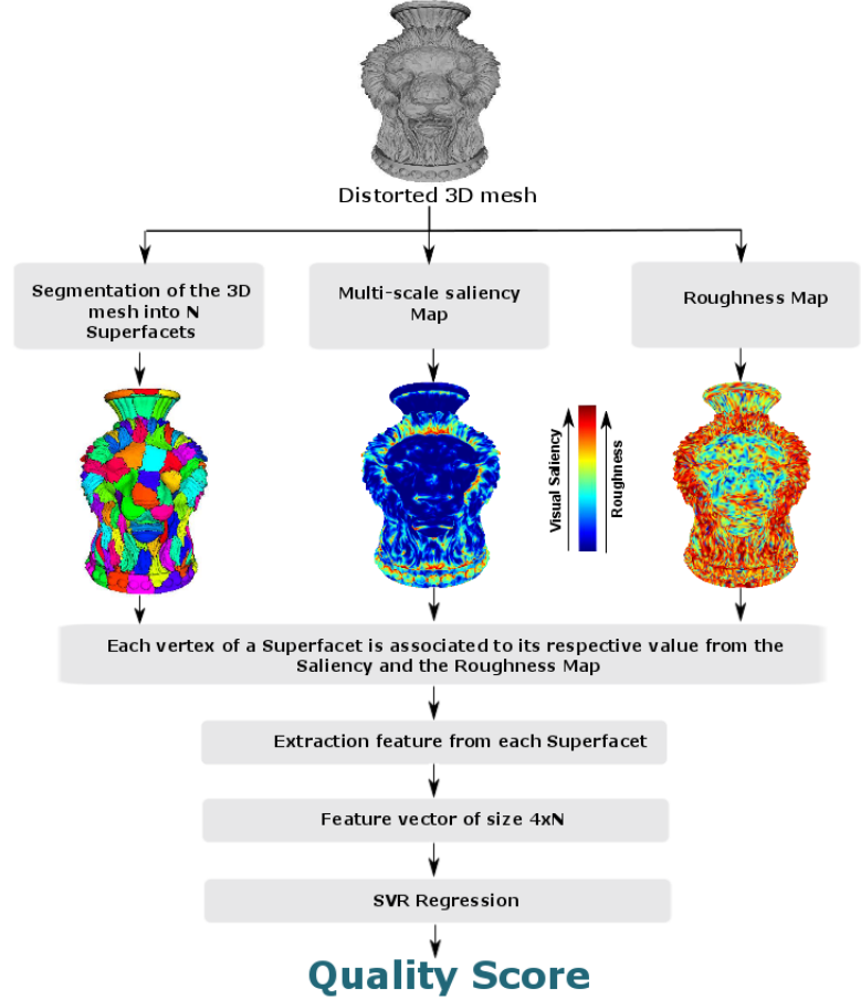
Figure 1: Block diagram of our metric
