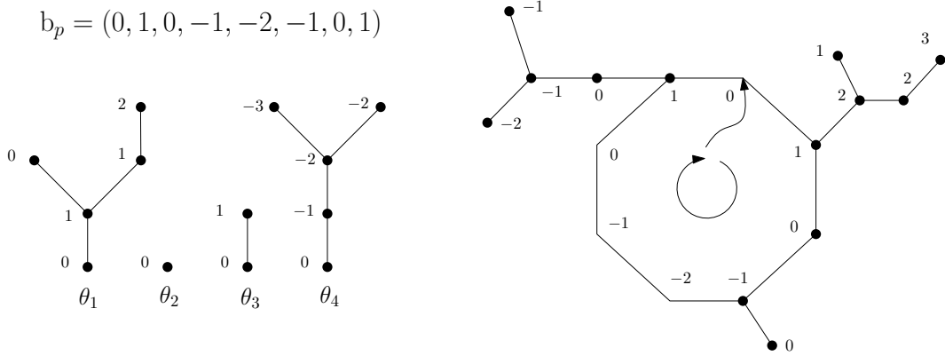
Figure 6: A labeled finite treed bridge and a representation of it. The black dots represent the vertices of the trees of the treed bridge.
