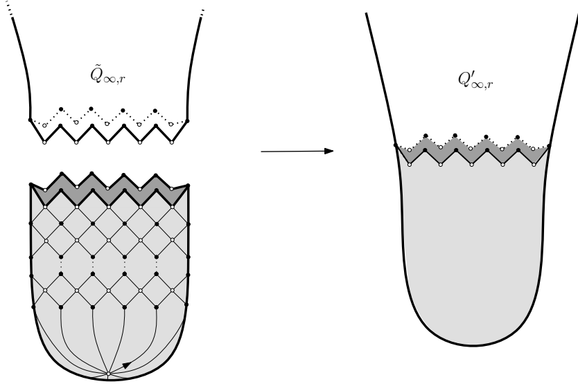
Figure 11: The filling operation.
