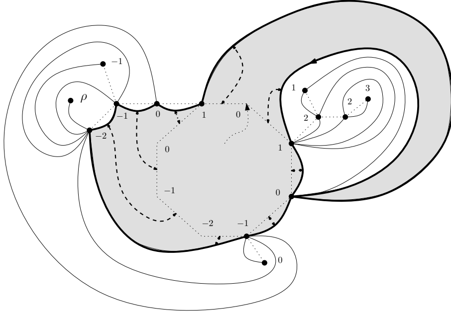
Figure 7: Construction of the rooted and pointed quadrangulation with a boundary associated with a treed bridge. The treed bridge is represented in dotted lines, the quadrangulation in solid lines, its boundary in thick lines and finally the correspondence between the embedded cycle and the boundary of the map is highlighted with dashed lines.
