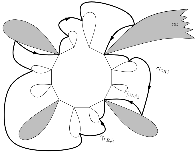
Figure 9: An illustration of the proof, the bad trees are represented in gray and the cycle constructed out of simple geodesics shortcutting them by a fat black line.
