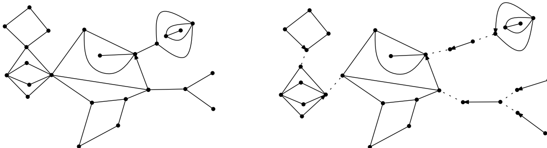
Figure 4: Decomposition of a quadrangulation with a boundary into irreducible components.
