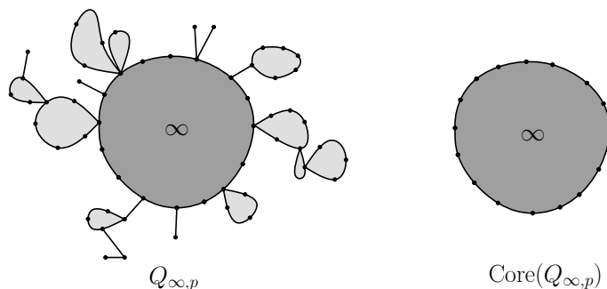
Figure 2: Pruning Q_{\infty,p} .
