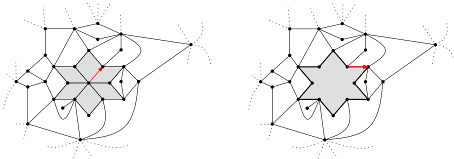
Figure 5: A fragment of a rooted quadrangulation with a special neighborhood of the root and the rooted quadrangulation with a simple boundary obtained by removing this neighborhood and transferring the root edge.
