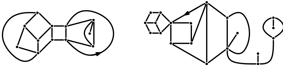
Figure 1: A quadrangulation with a simple boundary and a quadrangulation with a general boundary.
