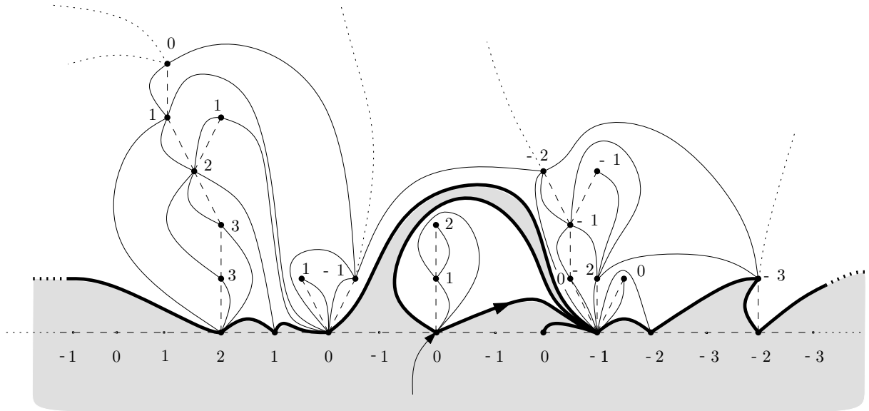
Figure 12: Second extension of \Phi . The infinite labeled treed bridge is represented with dashed lines, the map with solid lines and its boundary with thick lines.
