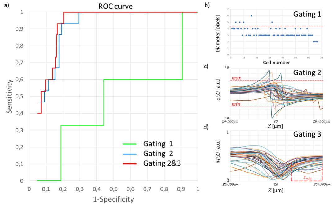
Figure 3. (a) Receiver operating characteristic (ROC) curves obtained with different lens-free classification algorithm for the detection of infectious meningitis. The green curve is obtained with a leukocytes count based on the measurement of the cell diameter. This gating is depicted in (b), a threshold (red dotted line) is applied to the distribution of the cell diameter in pixels ( 1.67\ \mu\text{m} pixel pitch). This threshold has been varied to compute the green ROC curve in (a). The blue ROC curve in (a) corresponds to the classification obtained with a gating applied to the phase Z -axis profiles measurement (Fig. 2h). This gating is depicted in (c). It selects phase Z -axis profiles of which the amplitude is larger than a defined threshold (red dotted line). The red ROC curve in (a) corresponds to the classification obtained with the phase gating and a module gating. The module gating is depicted in (d). It selects module Z -axis profiles (Fig. 2j) of which the local minima Z_{\text{min}} is well above the Z_0 .
