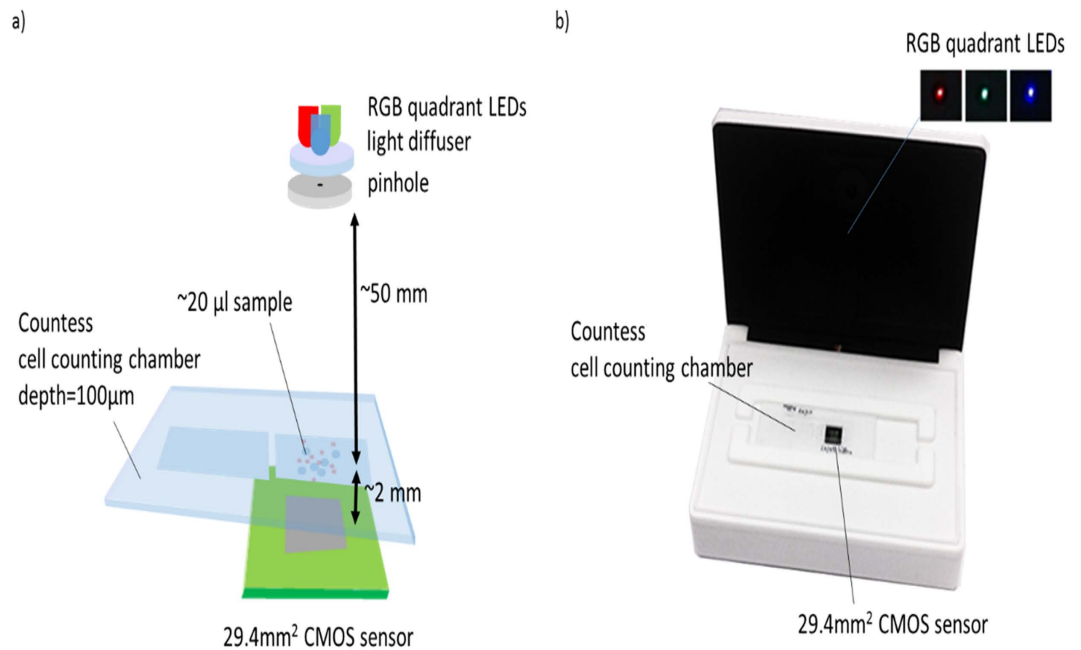
Figure 1. Experimental setup for the lens-free analysis of CSF clinical specimen. (a) Schematic of the optical setup. The multispectral illumination is provided by a multi-quadrant RGB LED coupled to a 150\mu\text{m} pinhole through a 60^\circ diffuser. When the quadrant RGB LED sequentially illuminates the sample, the CMOS sensor records three red, green and blue holograms. (b) Picture of the prototype used in the proof of concept study. The device cover featuring the RGB illumination is shown open in the picture.
