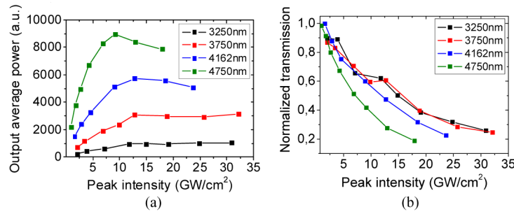
Fig. 4. (a) Output power from the Si/SiGe waveguide as a function of the coupled peak intensity for all the wavelengths used in the experiments. (b) Normalized transmission as a function of the coupled peak intensity.
