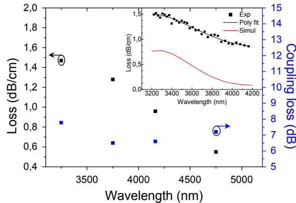
Fig. 2. Propagation loss and coupling loss as a function of wavelength for a waveguide with a cross section of 1.4 \times 2 \mu\text{m}^2 . In the inset the propagation loss of a waveguide with a 1.4 \times 1.9 \mu\text{m}^2 cross section is shown along with simulation results.
