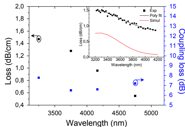
Fig. 2. Propagation loss and coupling loss as a function of wavelength for a waveguide with a cross section of 1.4 x 2 \mu\text{m}^2 . In the inset the propagation loss of a waveguide with a 1.4 x 1.9 \mu\text{m}^2 cross section is shown along with simulation results.
