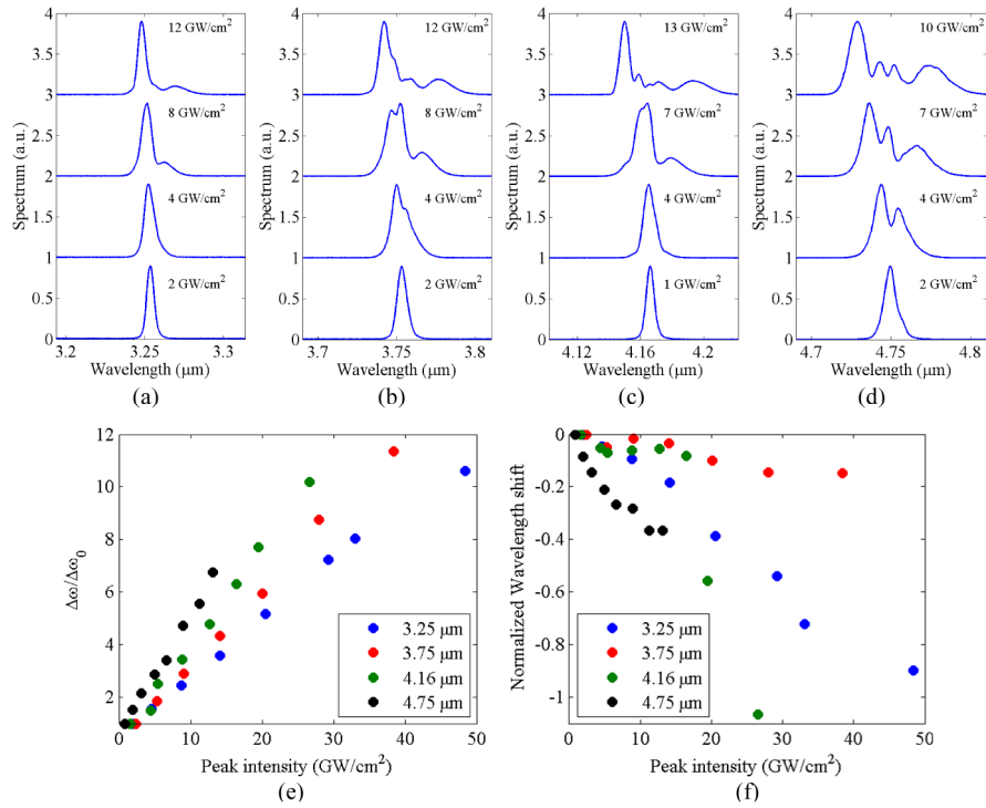
Fig. 3. (a-d) Normalized transmitted spectrum as a function of the coupled peak intensity for picosecond pulses centered at wavelengths between 3.25μm and 4.75μm. (e) and (f) Spectral broadening and normalized mean wavelength shift (i.e. (\lambda_c - \lambda_0)/\lambda_0 where \lambda_c is the mean wavelength of the spectrum and \lambda_0 is the low power mean wavelength) as a function the coupled peak intensity.
