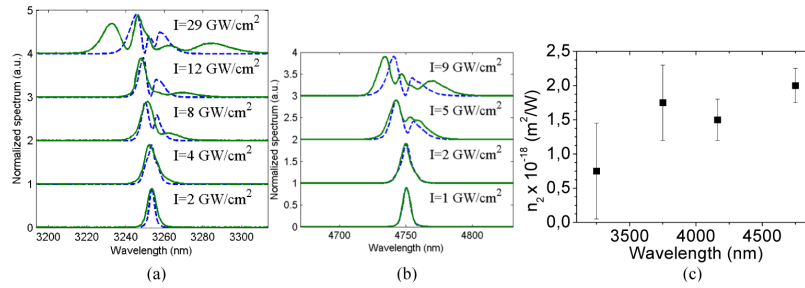
Fig. 6. Experimental (continuous line) and numerical (dashed line) transmission spectrum due to SPM as a function of the coupled peak intensity for a pulse centered at a wavelength of 3250 \text{ nm} , (a), and 4750 \text{ nm} , (b). (c) Nonlinear refractive index as a function of wavelength.
