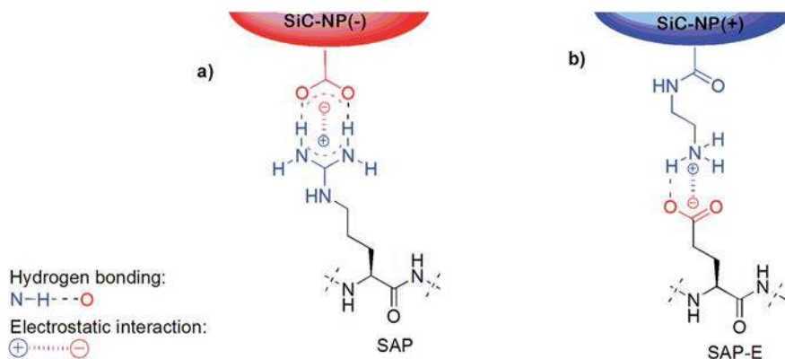
Fig. 2 Expected non-covalent interactions between oppositely charged SiC-NPs and CPPs. The as-prepared anionic SiC-NP(−) interacting with arginine side chains of SAP (a); and cationic SiC-NP(+) interacting with glutamate residues of SAP-E (b).
