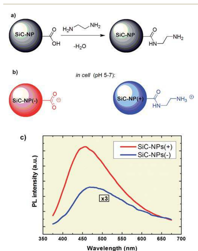
Fig. 1 Chemical modification of the carboxylic groups on the surface of the SiC-NPs (a), their ionization states under cellular internalization conditions (b), and photoluminescence spectra (excitation at 343 nm) of the as-prepared SiC-NPs used in this study (c).
