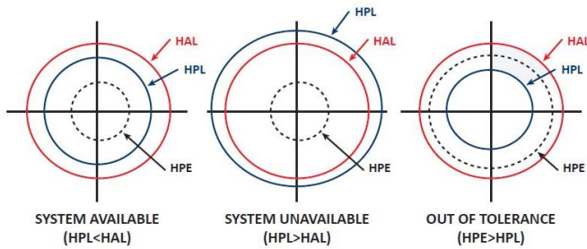
Fig. 14. Possible situations when navigating with EGNOS [77].
