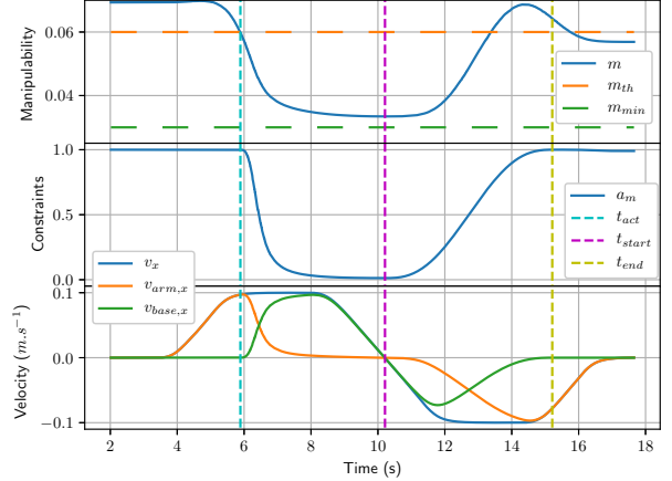
Fig. 3: Manipulability simulation. Top: manipulability measure m , middle: manipulability constraints a_m = a_{m,v_x} = a_{m,v_y} = a_{m,\omega_z} , bottom: Velocity commands along the x axis. t_{act} is the time at which the constraint gets activated.
