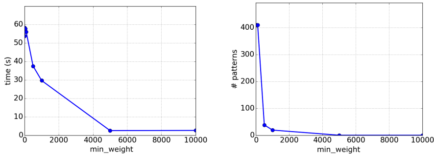
Fig. 20 Run times (left) and number of patterns (right) on VÉLO'V when varying min_weight .
