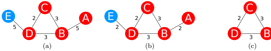
Fig. 1 Example of contextual subgraph and exceptional contextual subgraph: (a) Contextual graph associated to the most general context (*, *, *, *, *) = (Age \in [20, 50], Gender \in \{F, M\}, Time \in \{Day, Night\}, Weather \in \{Sunny, Cloudy, Windy, Rainy\}, type\ of\ area \in \{Bars, Residential\}) ; (b) A contextual subgraph of bike trips made by young people at night (Age \in [20, 23], *, Time \in \{Night\}, *, *) ; (c) An exceptional contextual subgraph with context (Age \in [20, 23], *, Time \in \{Night\}, *, type\ of\ area \in \{Bars\}) .
