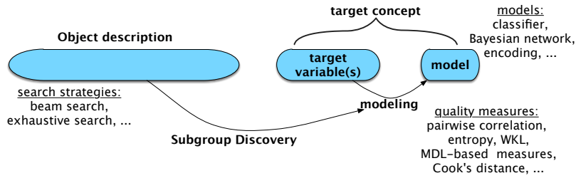
Fig. 2 The Exceptional Model Mining framework (diagram adapted from [15]).
