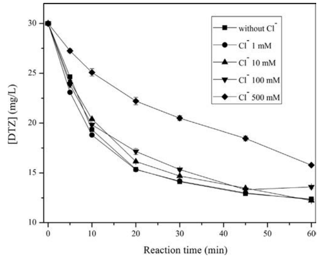
Fig. 7. Decomposition of DTZ by simulated sunlight activated PS in the presence of chloride. ([DTZ] 0 = 30 mg L -1 , [PS] 0 = 12 mM, initial pH = 6.5, reaction time = 60 min).
