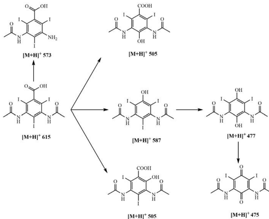
Fig. 4. Proposed oxidation pathways of DTZ by simulated sunlight activated PS. ( [DTZ]_0 = 30 \text{ mg L}^{-1} , [PS]_0 = 12 \text{ mM} , \text{pH} = 6.5 , reaction time = 60 min).
