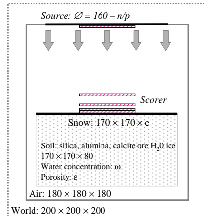
Fig. 3: Description of the modeled scene from GEANT4. The elementary volumes representing the atmosphere, soil and snow are represented. The particle generation disc is also visible at the top of the atmosphere. The cylindrical volumes sensitive samplings at different altitudes are also presented (dimensions in meter).
