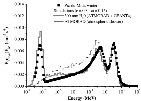
Fig. 10 : Neutron spectrum issued from measurements (winter) and simulation (ATMORAD + GEANT4 ground albedo neutron) considering a porosity of 0.30 a wet rocks of 15 % and a liquid water layer with a thickness of 300 mm.
