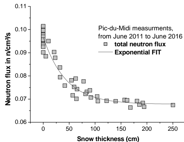
Fig. 5 : Neutron flux recorded from June 2011 to June 2016 in the Pic-du-Midi, versus the averaged thickness of accumulated snow in the Pyrenees (measured closed to the Pic-du-Midi station).
