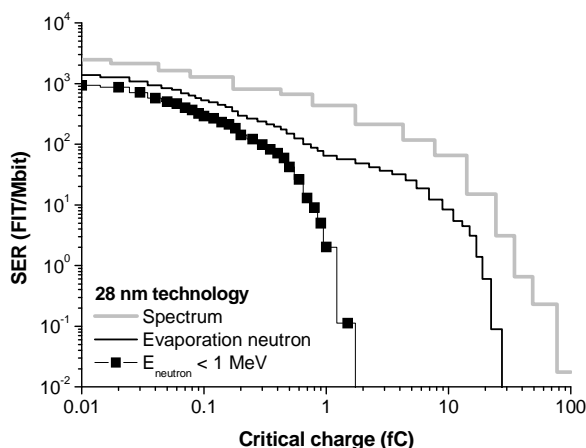
Fig. 11 : Predicted FIT rate for the 28 nm bulk CMOS cell considering neutron spectrum in ground and allowing to distinguish contributions induced by evaporation neutron (< 20 MeV) and by neutron energy less than 1 MeV.
