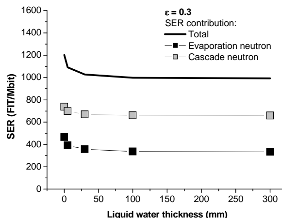
Fig. 13 : Predicted failure rate as function of the liquid water thickness, considering the neutron spectrum in ground (ATMORAD), and allowing to distinguish the evaporation contribution and the cascade contribution.
