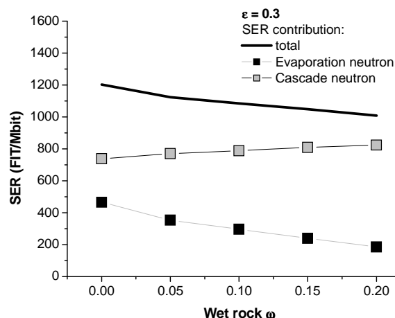
Fig. 12 : Predicted failure rate as function of the wet rock fraction, considering the neutron spectrum in ground (ATMORAD), and allowing to distinguish the evaporation contribution and the cascade contribution.
