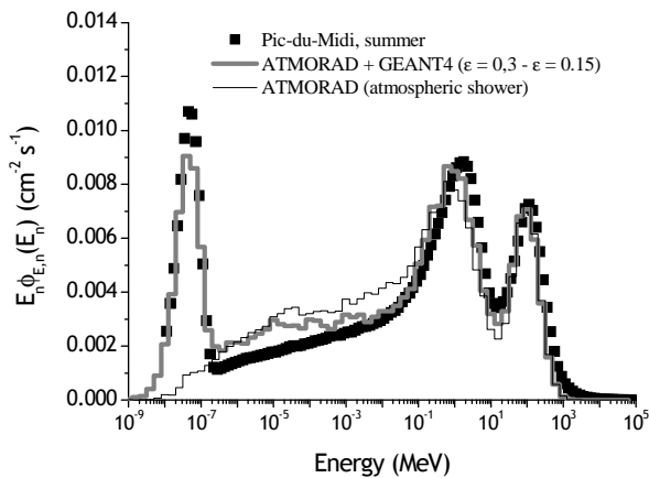
Fig. 8 : Neutron spectrum issued from measurements (summer) and simulation (ATMORAD + GEANT4 ground albedo neutron) considering a porosity of 0.30 and wet rocks of 15 %.
