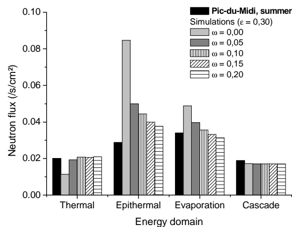
Fig. 7 : Neutron flux in 1/s/cm 2 for each energy domain. Comparison between measurements and simulations considering a porosity of 0.30 and various wet rocks from 0 to 20%.
