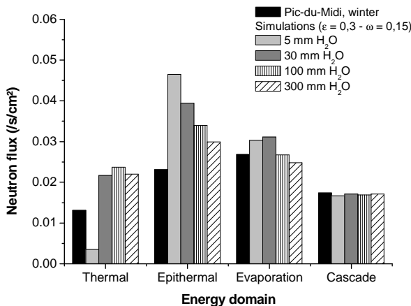
Fig. 9 : Neutron flux in /s/cm 2 for each energy domain. Comparison between measurements and simulations considering a porosity of 0.30, a wet rocks of 15 % and for various liquid water layers with a thickness from 5 to 300 mm. The experimental spectrum given by the spectrometer during winter is plotted.
