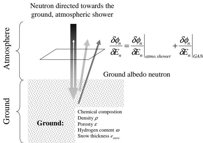
Fig. 2: Overview of the approach, the neutron spectrum result from the sum of atmospheric spectrum deduced from ATMORAD and ground albedo neutron calculated thanks to GEANT4 simulations.
