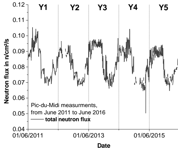
Fig. 4 : Neutron flux variations from June 2011 to June 2016 in the Pic-du-Midi.
