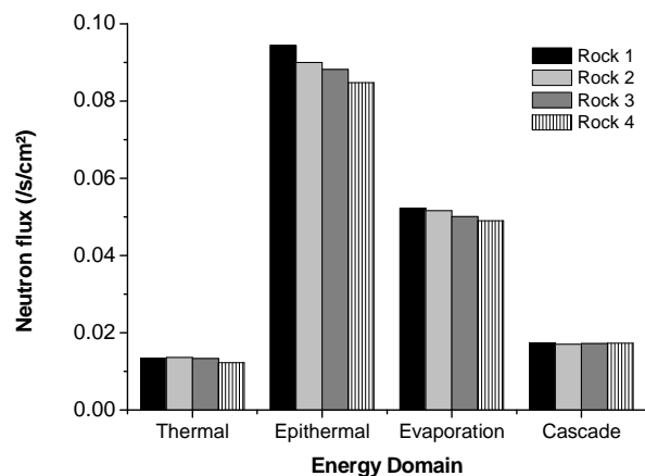
Fig. 6 : Neutron flux in 1/s/cm 2 for each energy domain, GEANT4 results obtained for 4 rocks chosen for their chemical composition.
