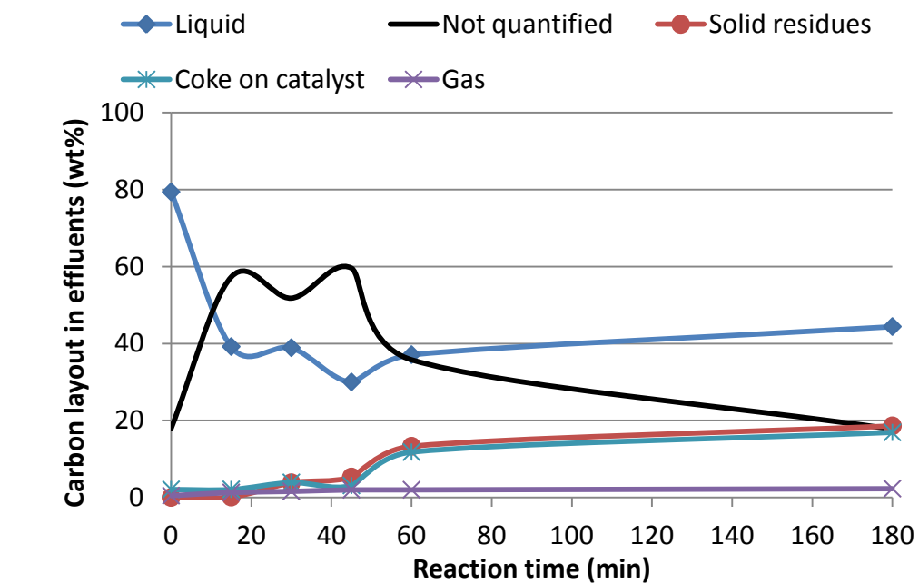
Figure 2 : [A] Experimental mass and [B] carbon balances of Mixture A (Gua/Fur/AA/Glu) hydroconversion as function of time (250 °C)
