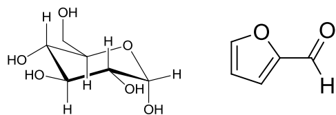
D-Glucose
