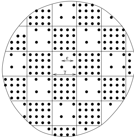
Fig. 2. The limiting process allowing the derivation of (62), with K = 2
