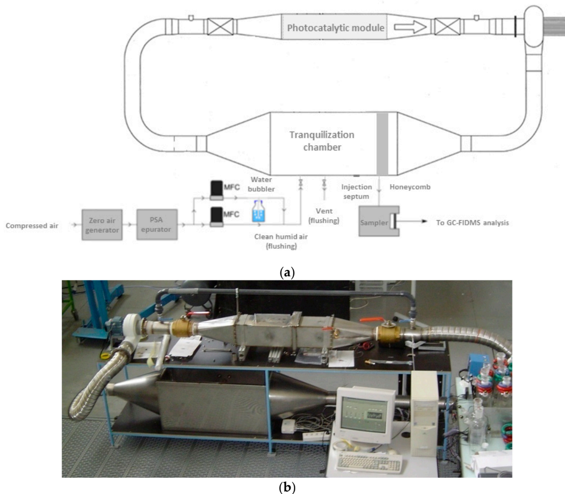
Figure 1. Experimental closed-loop reactor operating in recirculation mode. (a) Schematic representation; and (b) photograph of the whole system.
