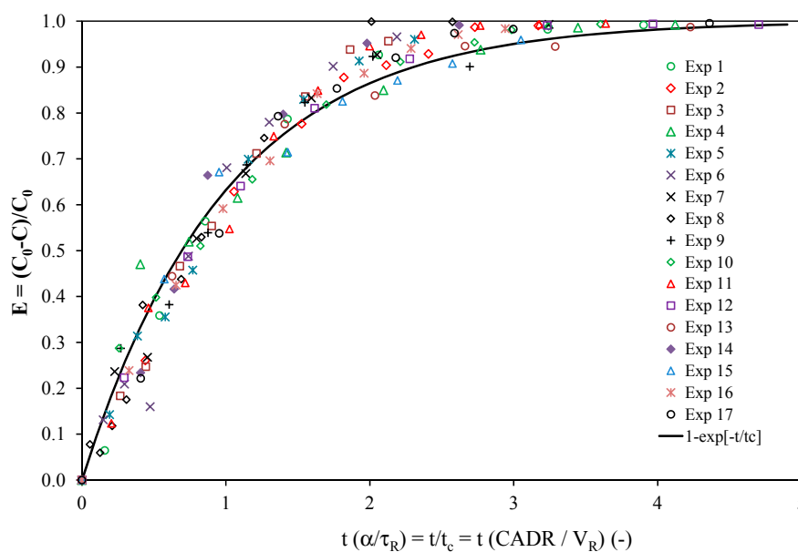
Figure 4. Toluene removal efficiency for all experiments according to the generalized form (Equation (4)).
