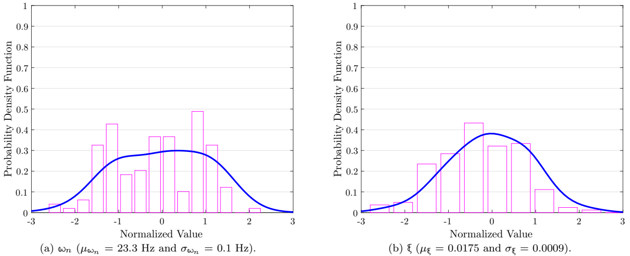
Figure 4: PDFs of the natural frequency and damping ratio of the equivalent linear system.
