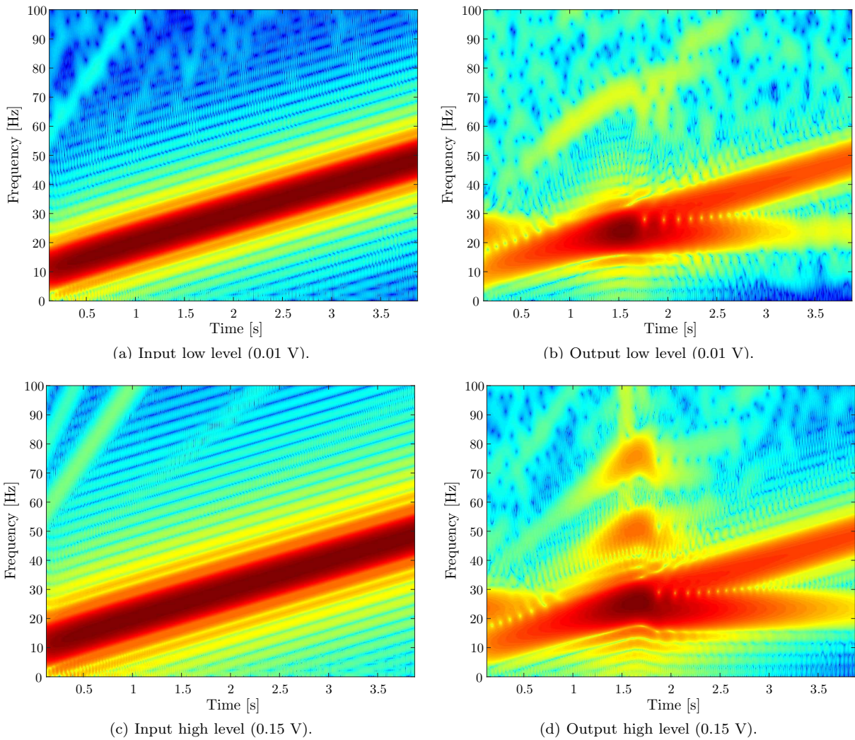
Figure 3: Spectrogram of the inputs and outputs considering different levels.
