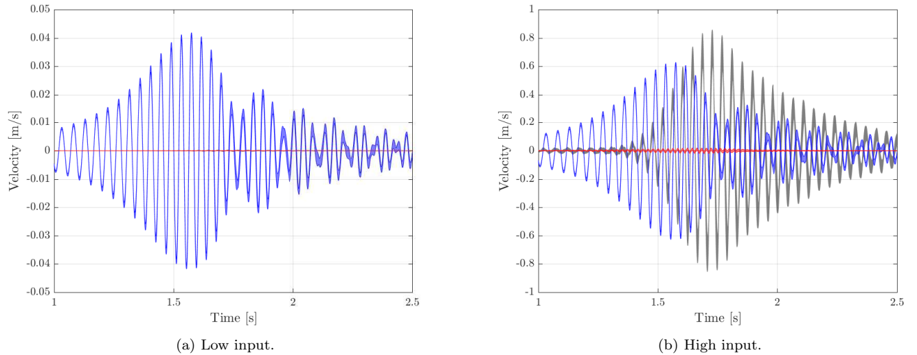
Figure 8: Confidence bands for the contributions to the system responses obtained through the Volterra model with 98 % of confidence. ■ represents the linear contribution, ■ represents the quadratic contribution and ■ represents the cubic contribution.
