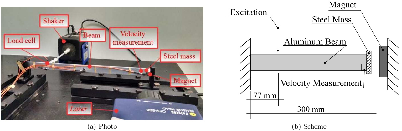
Figure 1: Experimental setup.
