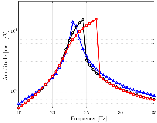
Figure 2: Beam extreme velocity during a stepped sine test, where \triangle represents the low level of input signal (0.01 V), \circ the medium level (0.10 V) and \square the high level (0.15 V).
