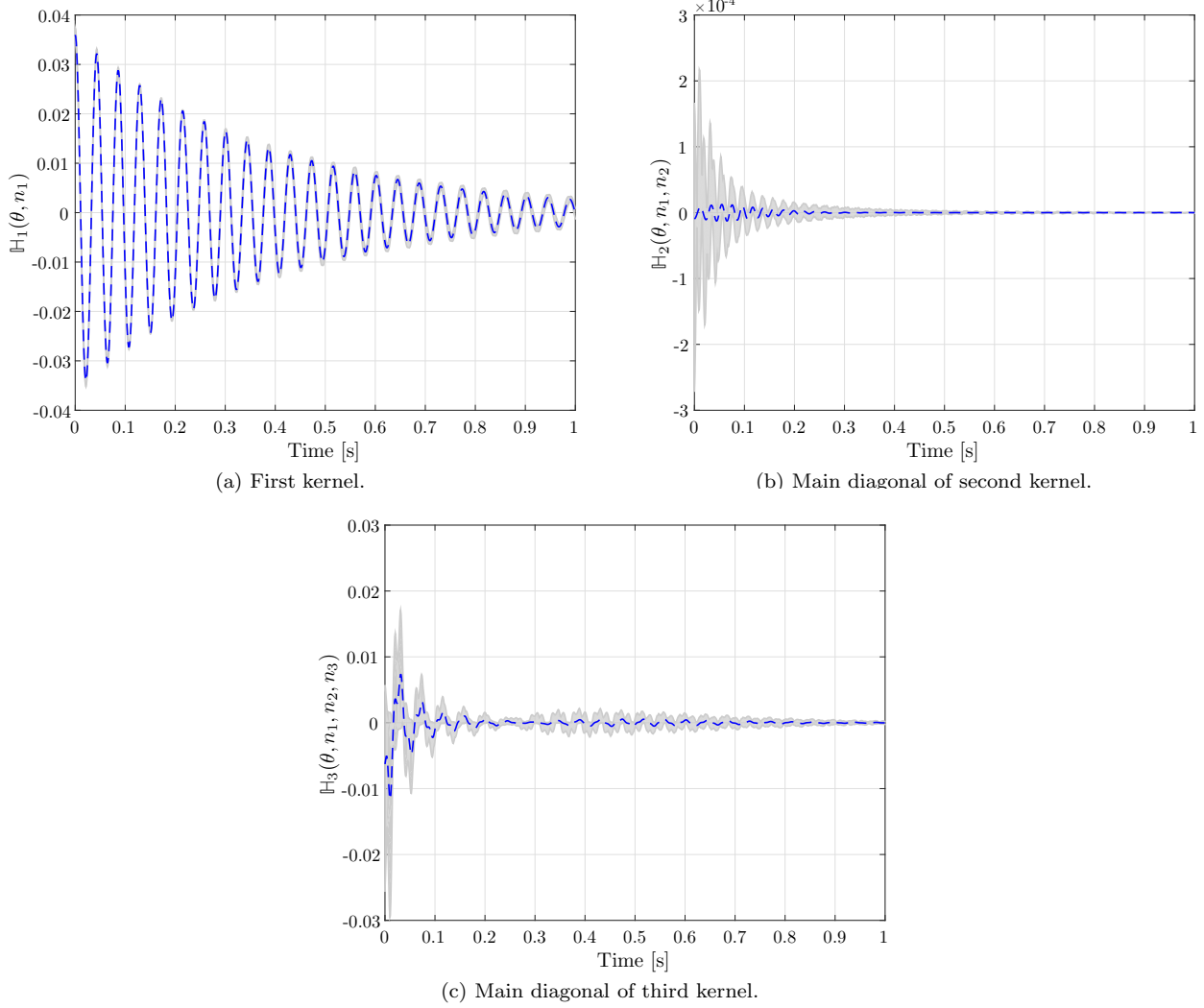
Figure 6: Volterra kernels limits with 98 % of confidence, the blue line represents the mean value.
