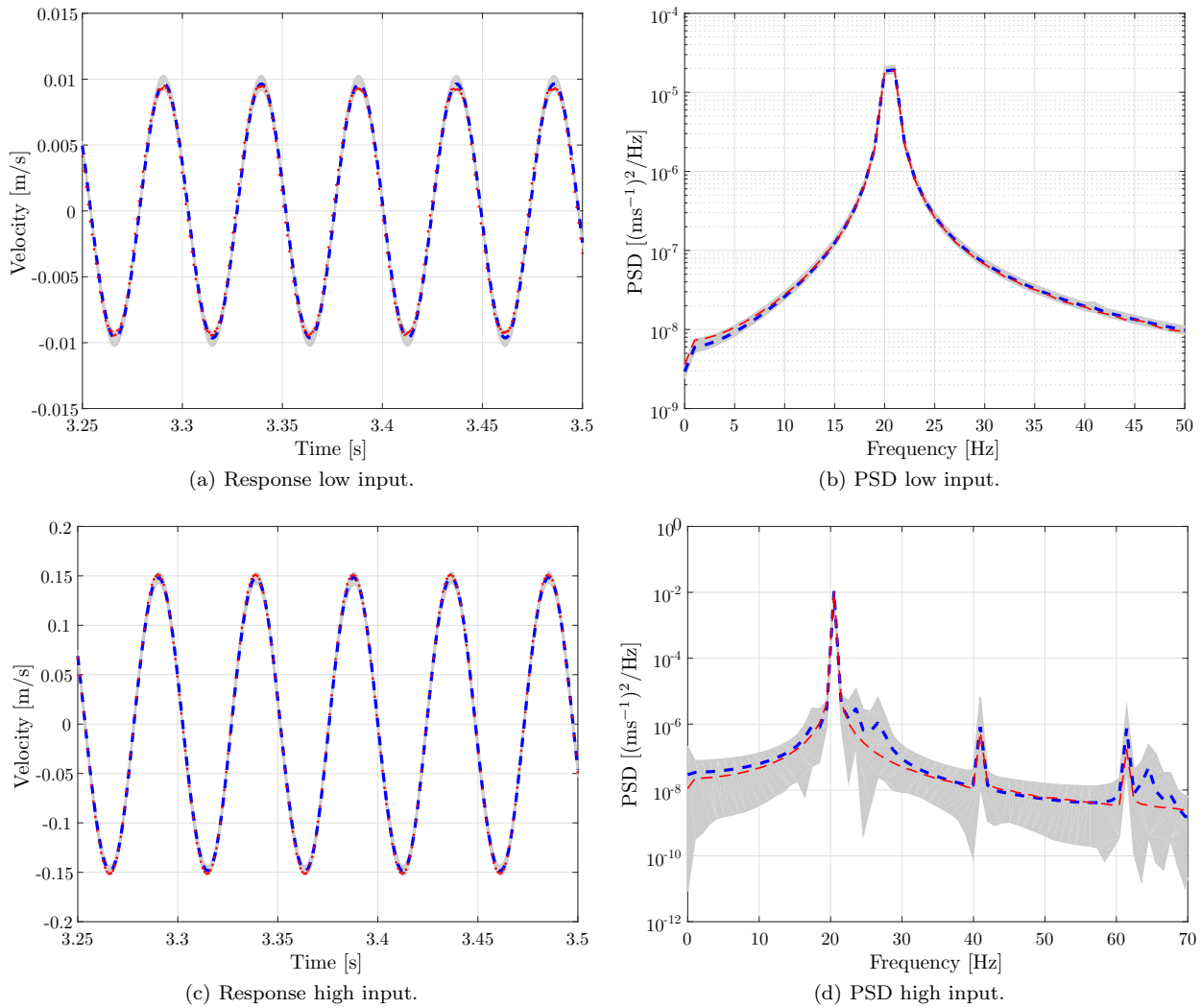
Figure 9: Confidence bands for the system responses obtained through the Volterra model with 98 % of confidence. The mean is represented by the blue line and the experimental data are represented by the red line.
