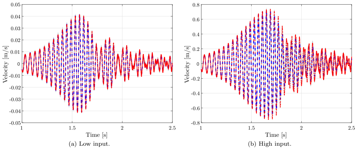
Figure 7: Confidence bands for the system responses obtained through the Volterra model with 98 % of confidence. The mean is represented by the blue line and the experimental data are represented by the red dots.
