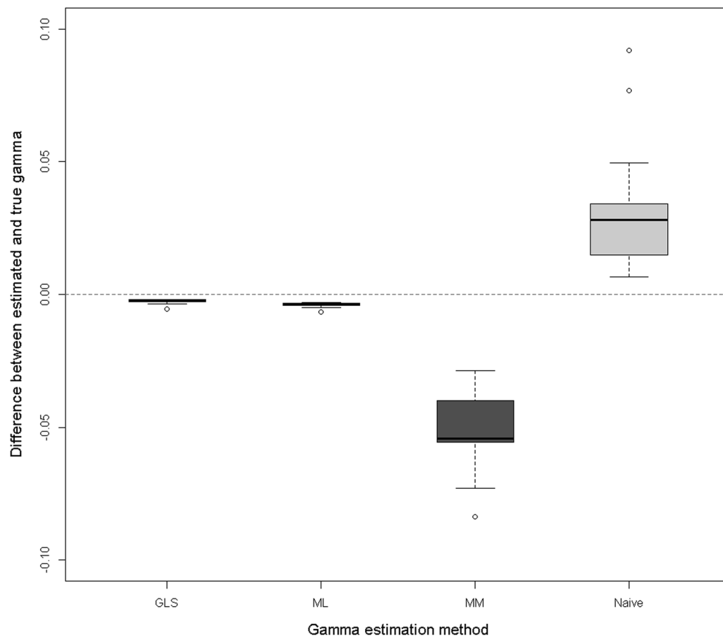
Fig. 1 Differences between estimated and true Gamma, across 20 simulation replicates. Gamma was estimated by generalized least squares (GLS), maximum likelihood (ML), method of moments (MM) and the Naive method
