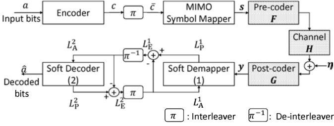
Fig. 1: System model.
