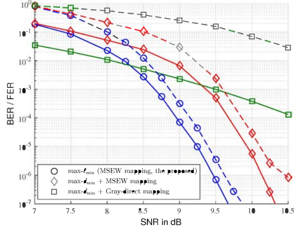
Fig. 7: Average BER (solid lines) and FER (dashed lines) performance of the precoded turbo detection over random 2 \times 2 MIMO channels.
